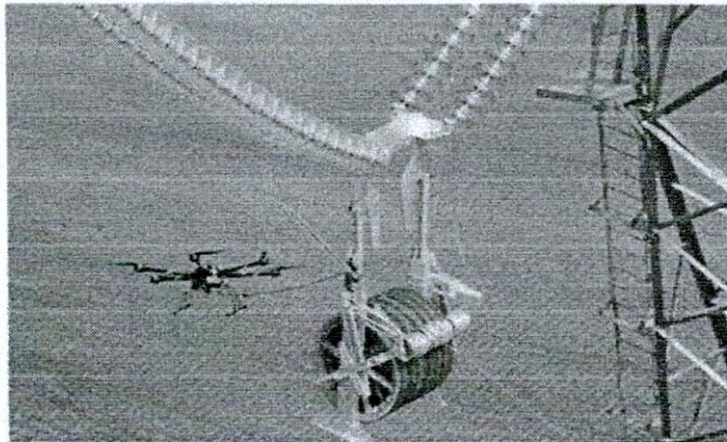
Fig 2.3: Conductor Stringing
