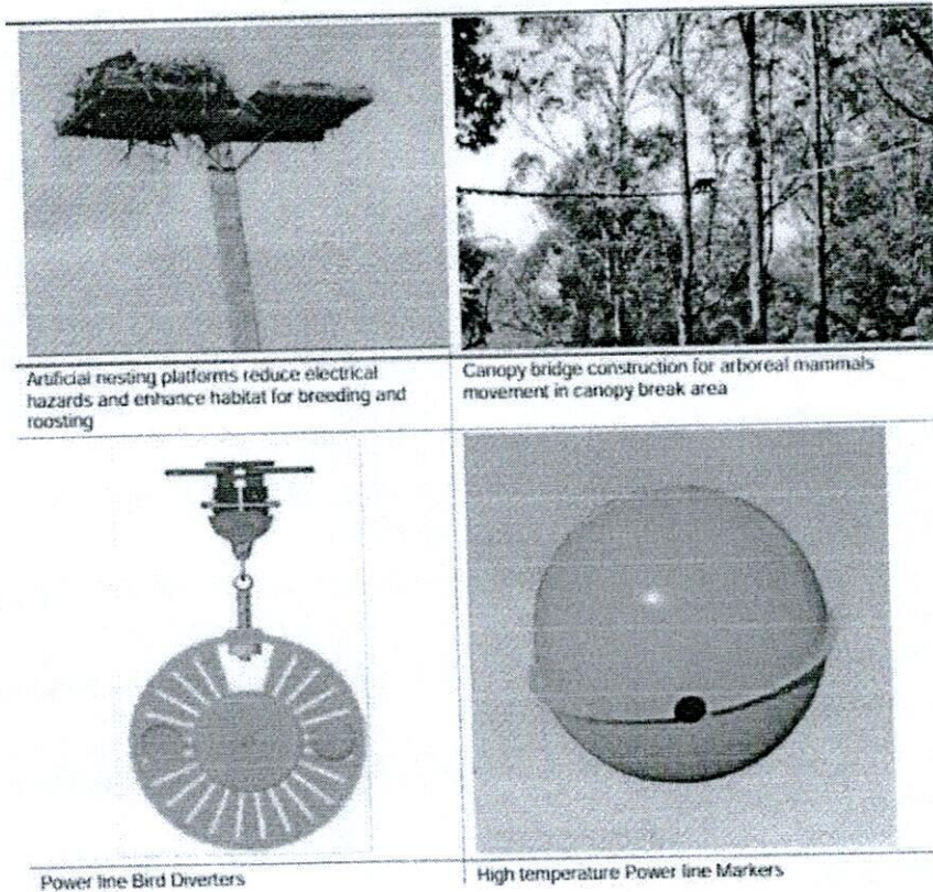
Fig 3.1: Mitigation Structures for Transmission Line
