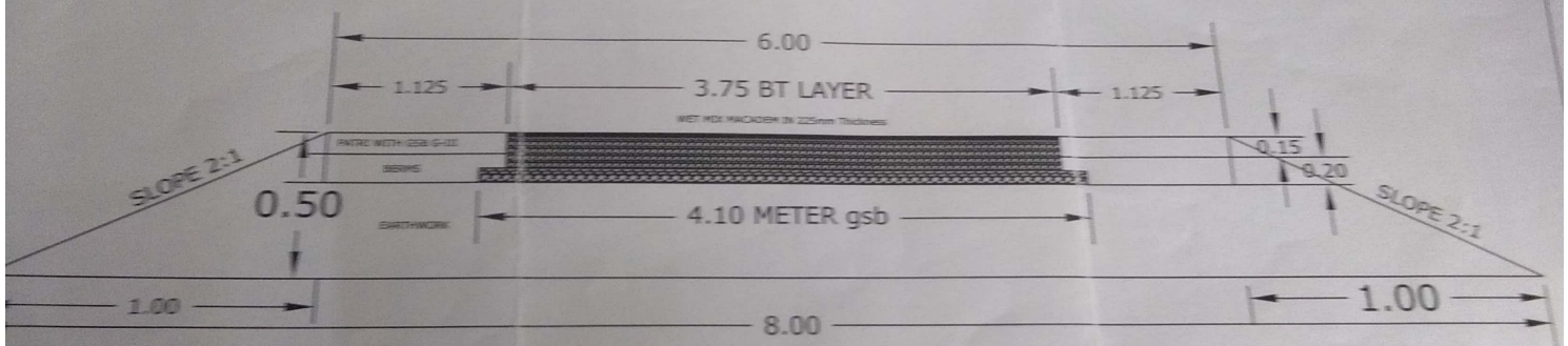
PROPOSED X-SECTIONAL MAP OF ROAD
