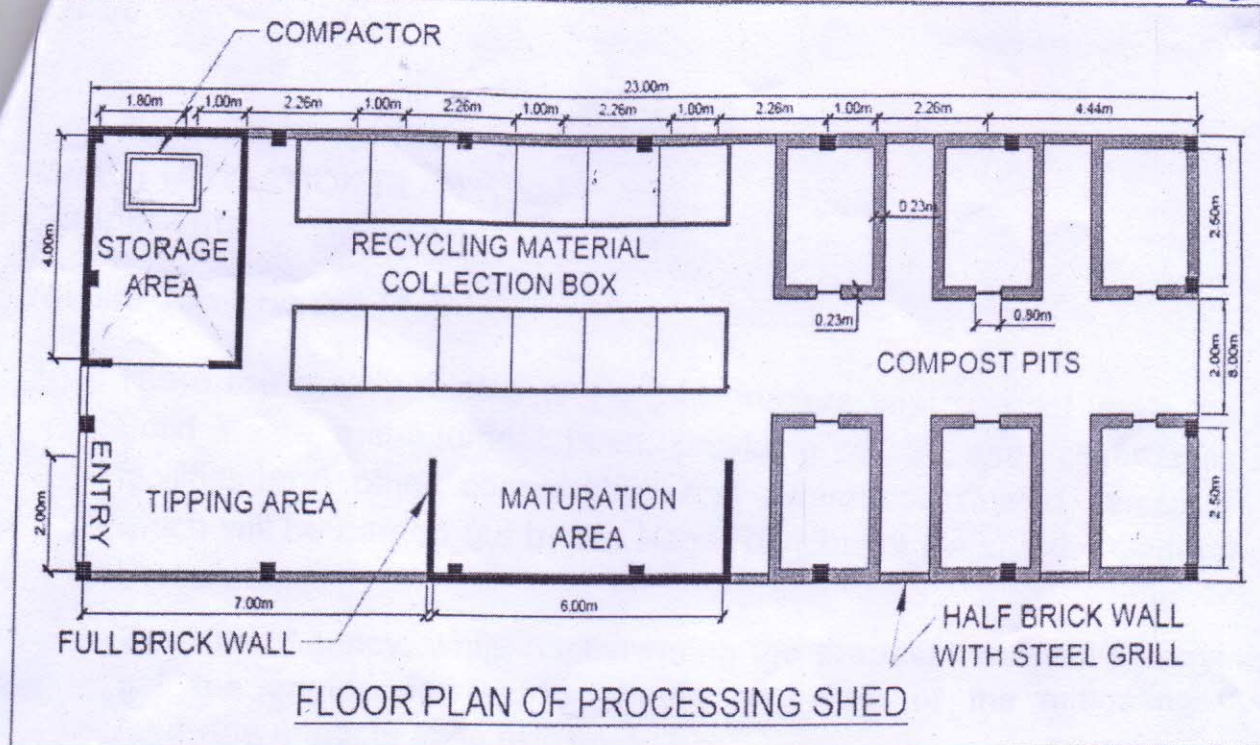
Fig. Layout of the tipping & plastic segregation shed
