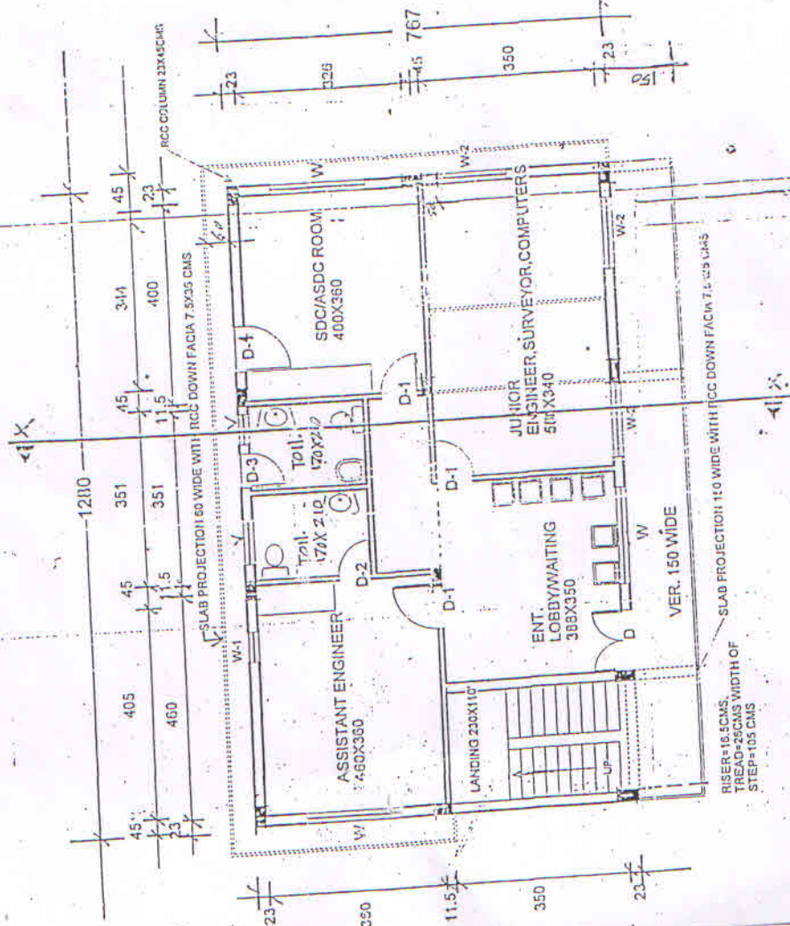
PLAN AT LEVEL -1 FLOOR
