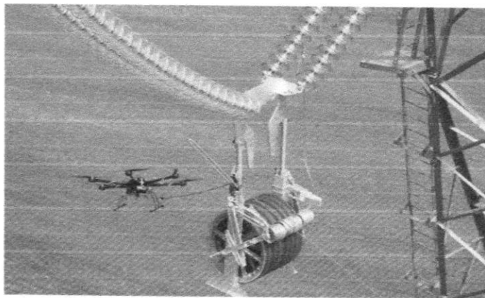
Fig 2.3: Conductor Stringing
