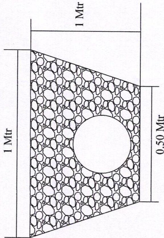
Cross Section
