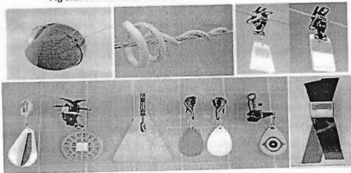
Fig 3.2: Bird Diverter/Coloured/Contrast Marker Devices
