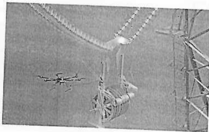
Fig 2.3: Conductor Stringing
