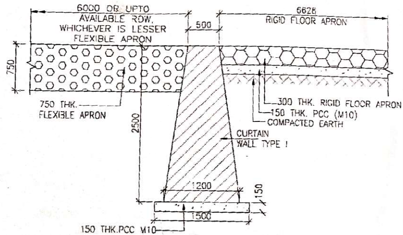
DETAIL OF CURTAIN WALL TYPE I TO BE PROVIDED ON DOWN STREAM (SCALE 1:50)
