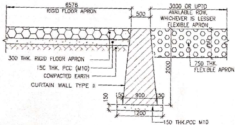
DETAIL OF CURTAIN WALL TYPE II TO BE PROVIDED ON UP STREAM (SCALE 1:50)
