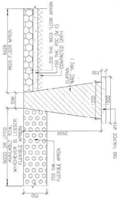
DETAIL OF CURTAIN WALL TYPE I TO BE PROVIDED ON DOWN STREAM (SCALE 1:50)
