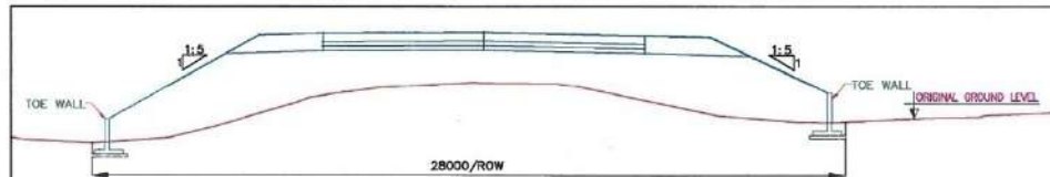
TYPICAL CROSS SECTION IN EMBANKMENT SCALE - 1:100
