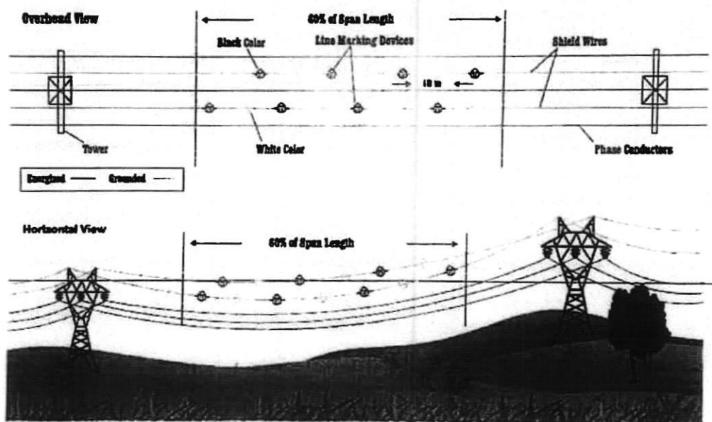
Figure 12.8: Design and configuration of markers to reduce bird collisions (after Eskom Transmission (South Africa) 2009). Source: APSC, 2012
