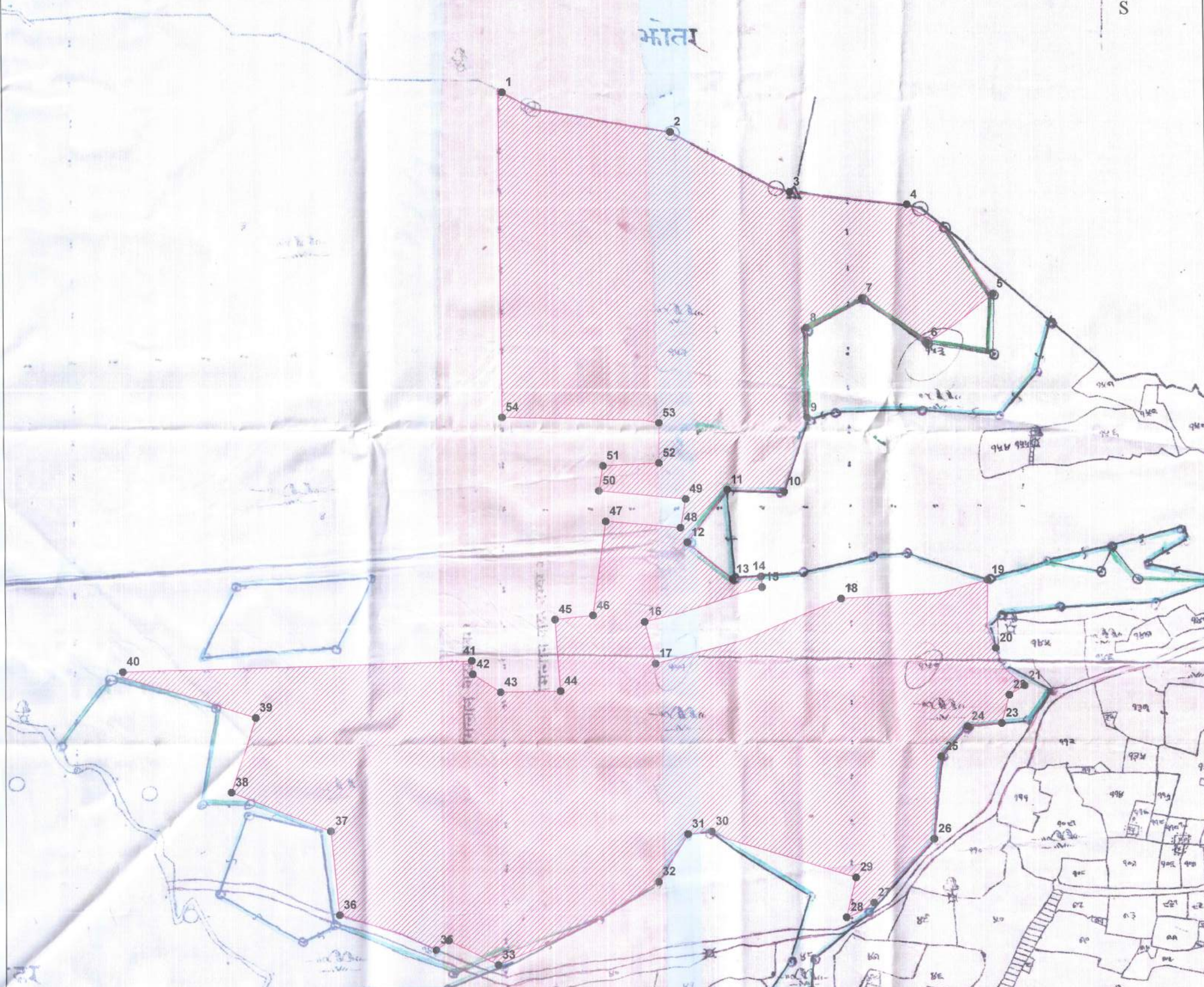
DGPS SURVEY CO-ORDINATES OF PILLAR POINTS Datum: WGS 84
