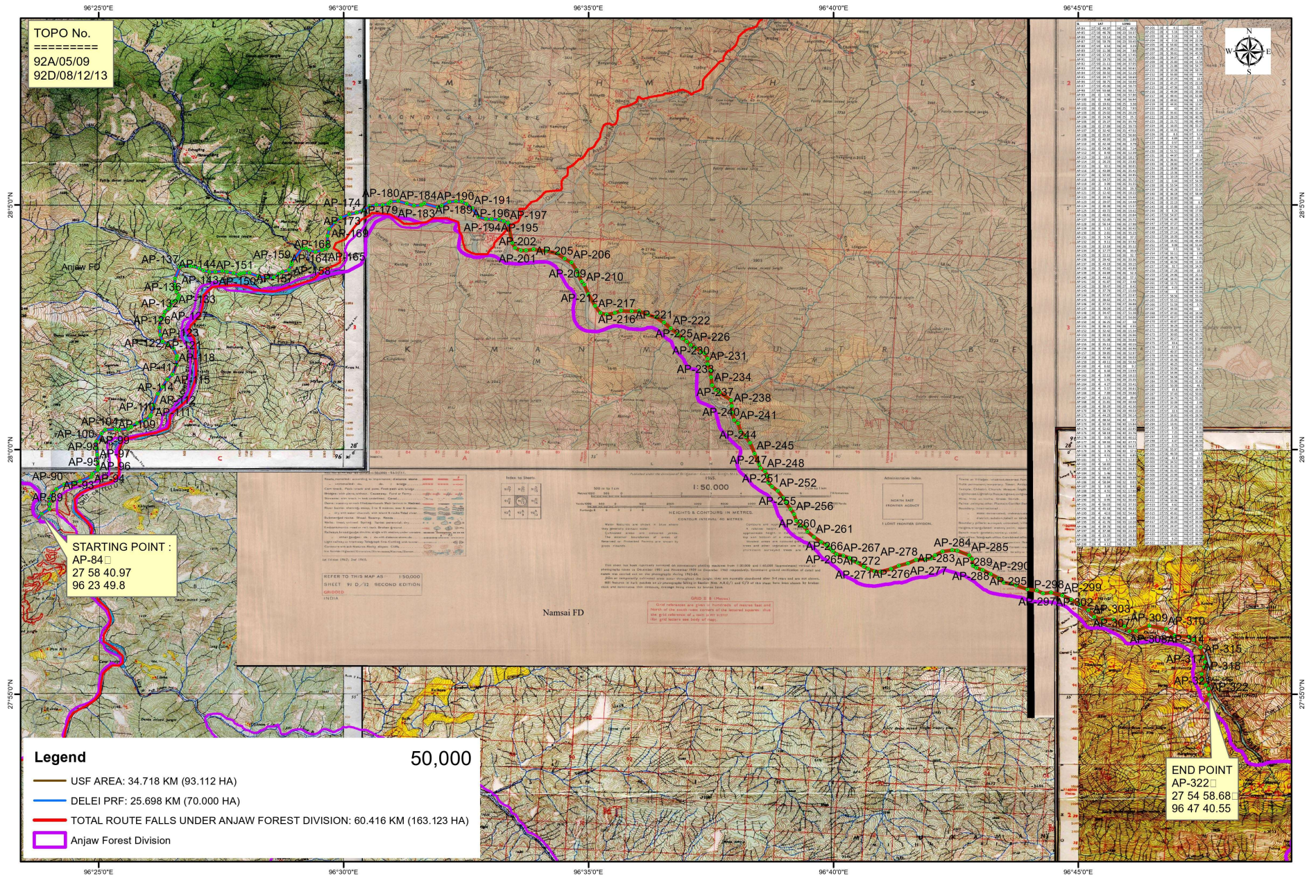
MAP SHOWING 132 KV T/L FALLS UNDER RESERVE FORESTS OF ANJAW FOREST DIVISION
