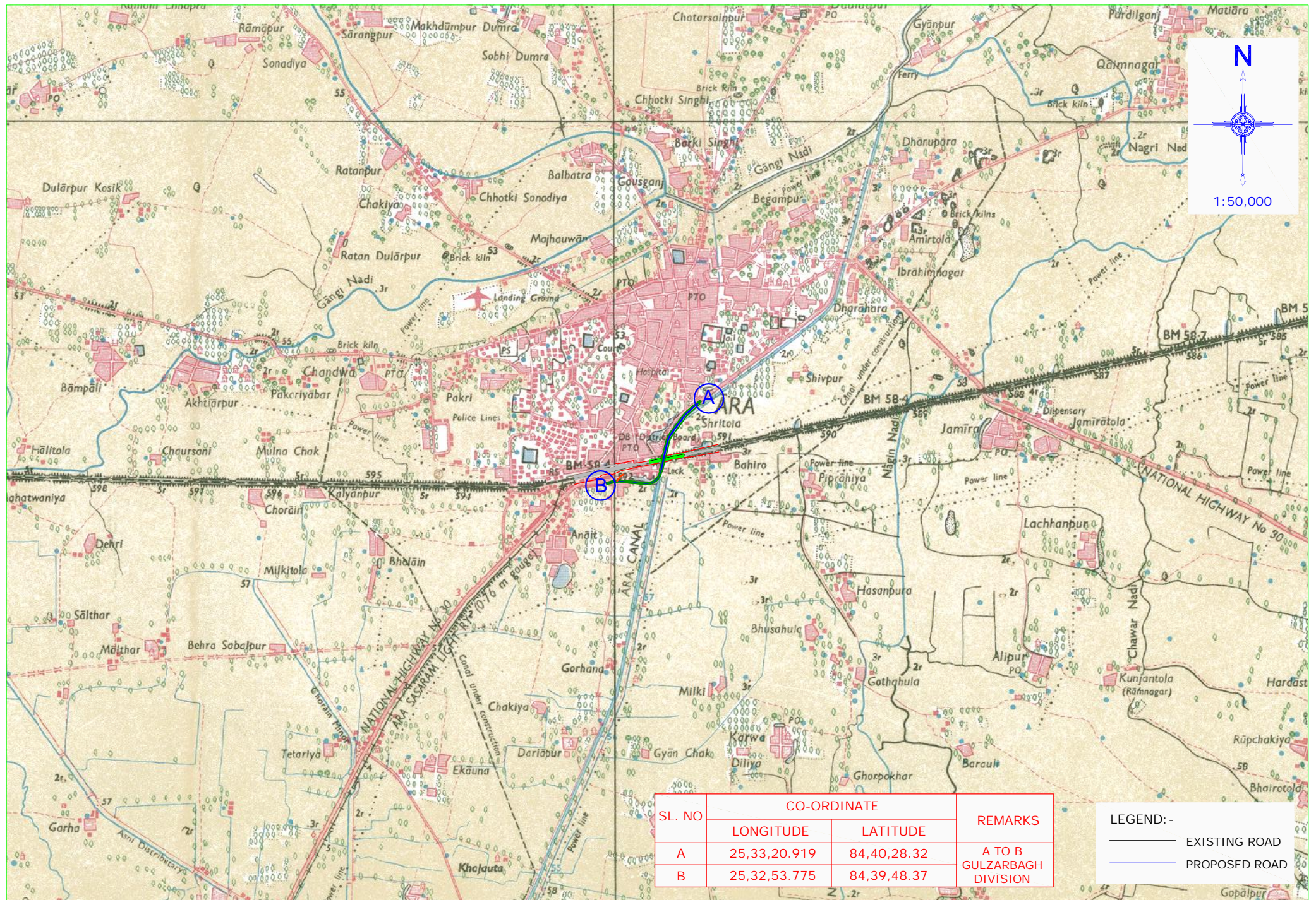
MAP SHOWING PROPOSED ALIGNMENT FOR ROB OVER L.C NO - 48A/31 AT CHAINAGE KM 118.089 TO KM 119.572
