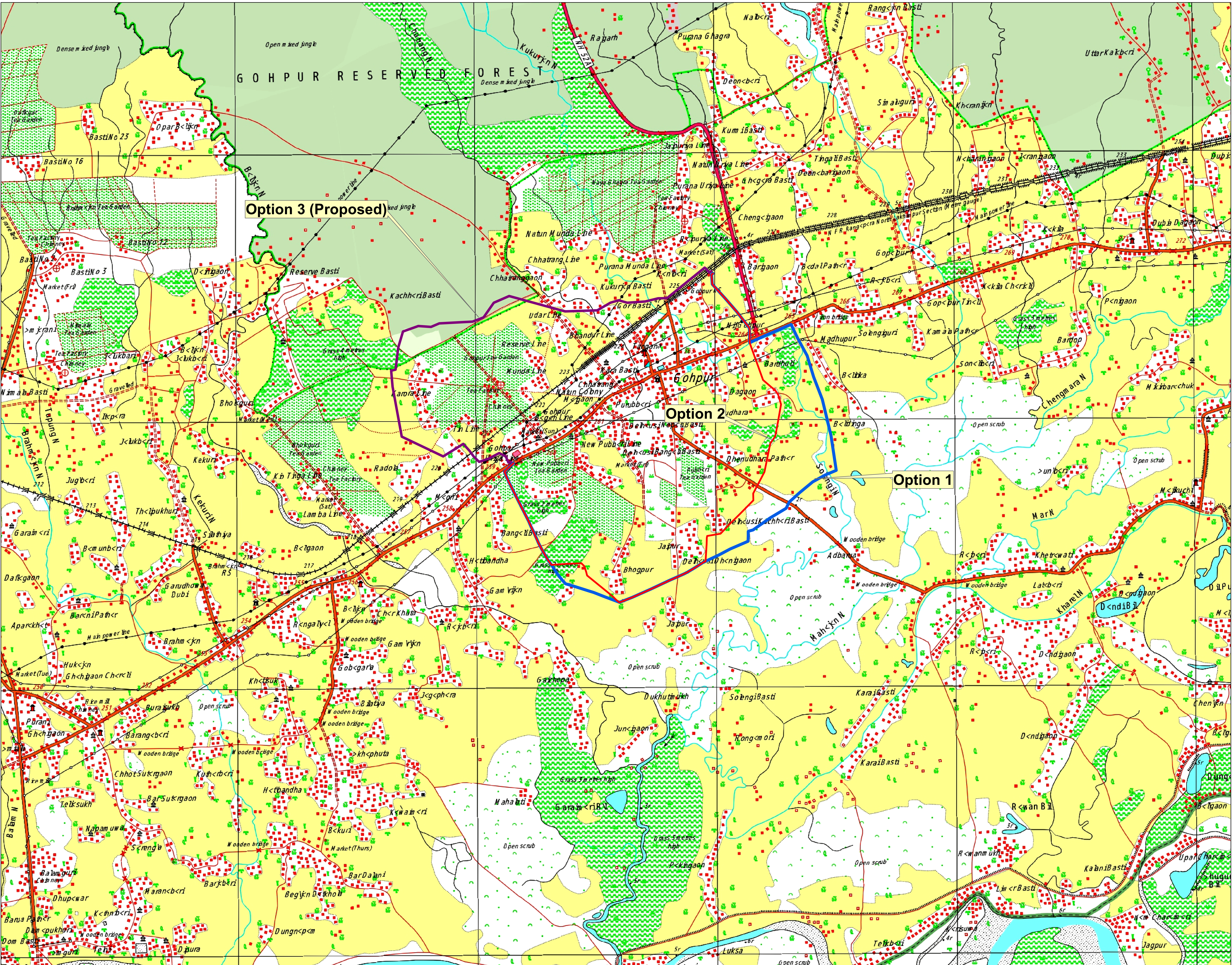
Map Showing 3 Alternative Routes of 132 KV EHT Single Circuit in connection with RNY-MZS Railway Electrification ProjectTransmission Line
