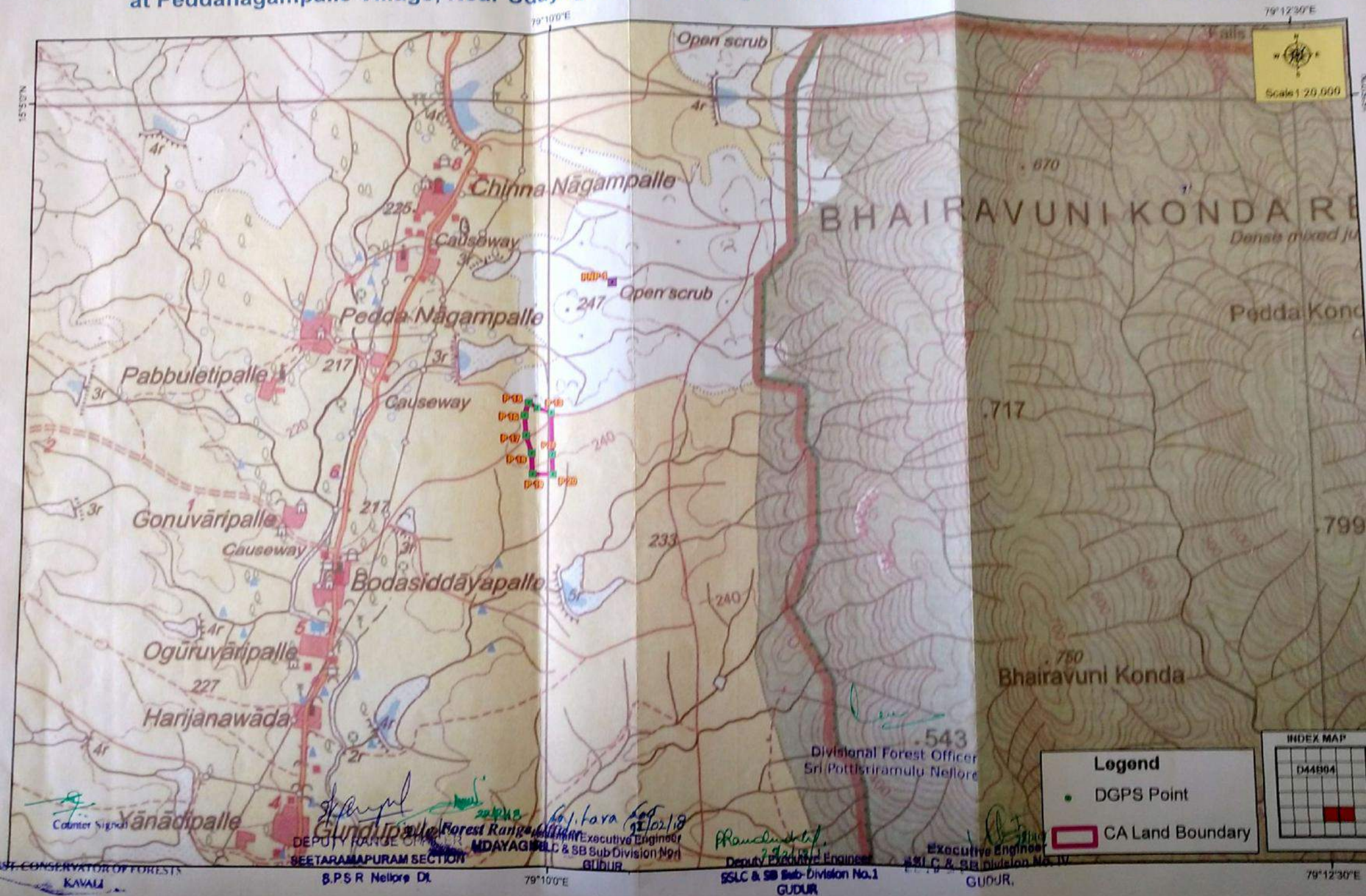
DGPS Survey Plan Showing the C.A. Land of 5.71 Ha of Somasila High Level Lift Canal Project Peddanagampalle Village, Near Udayagiri Forest Range of Nellore Forest Division, Nellore District.
