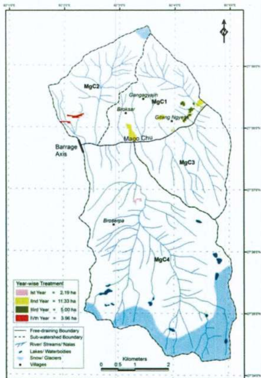
Figure 1-9: Year wise Treatment Index map for free draining catchment showing schedule of implementation measures
