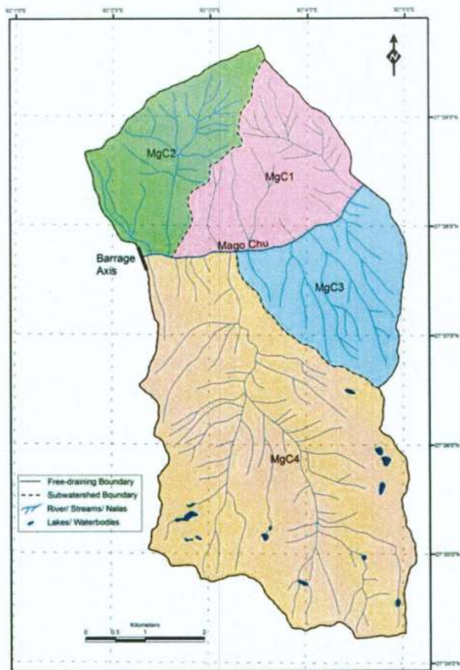
Figure 1-1: Index map of different sub- watersheds of free draining catchment
