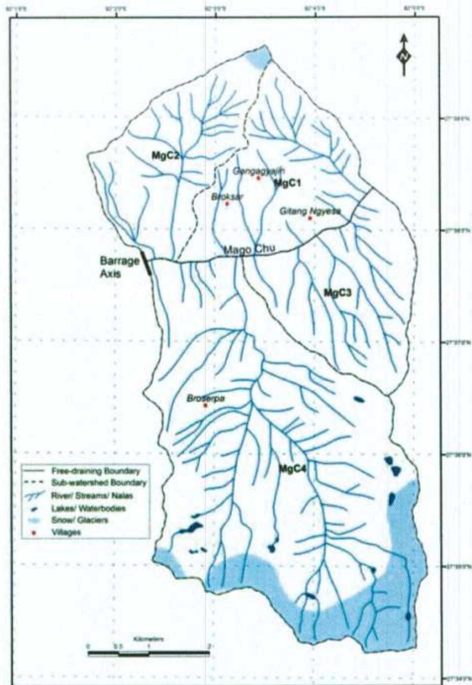
Figure 1-2: Drainage Map of Free Draining Catchment
