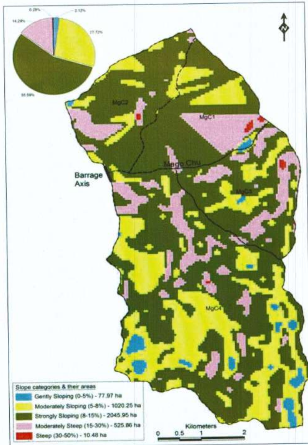
Figure 1-6: Slope Map of Free Draining Catchment
