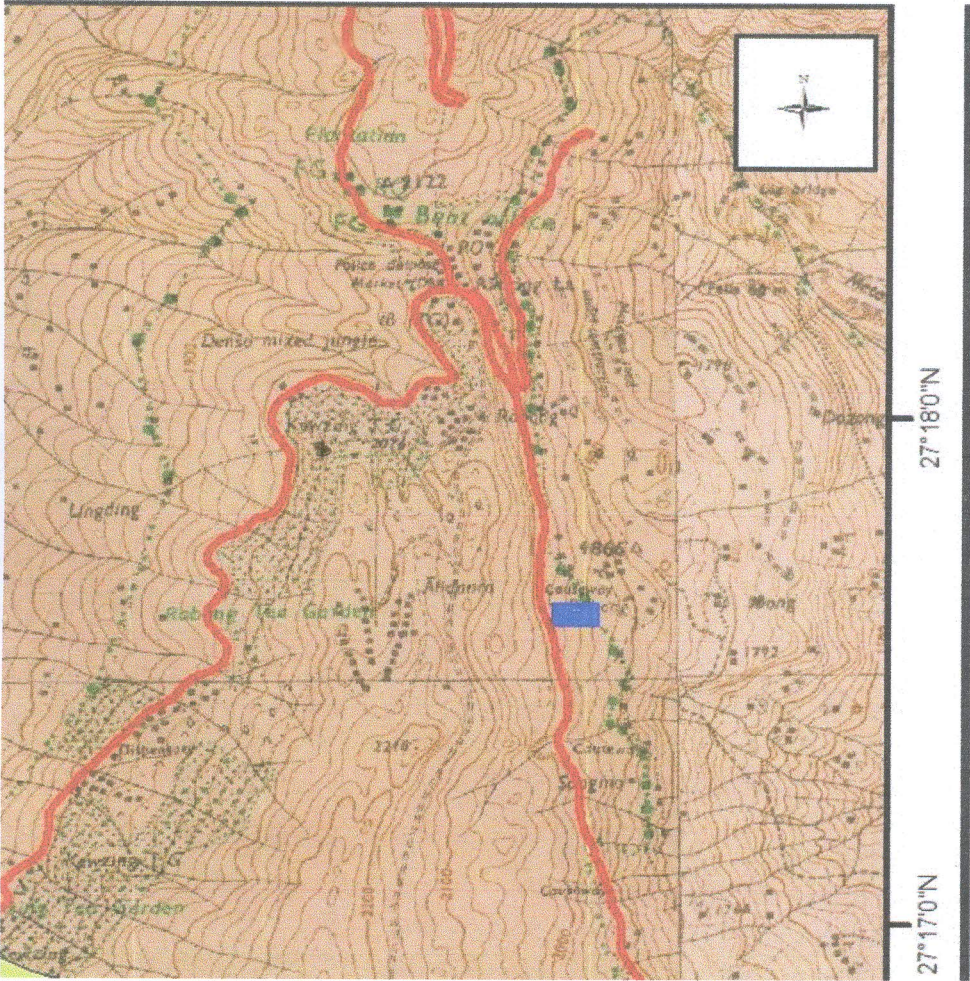
Map showing CAS for proposed work “Construction of 66 KVS/C Transmission line from 132/66 KV Switch Yard at Rabongla to Central University with 66/11 KV, 2X5MVA Substation at Yangang in South Sikkim.
