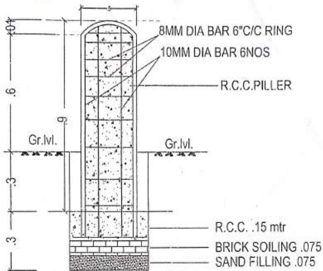
CROSS SECTION OF PILLER UNIT IN METER
