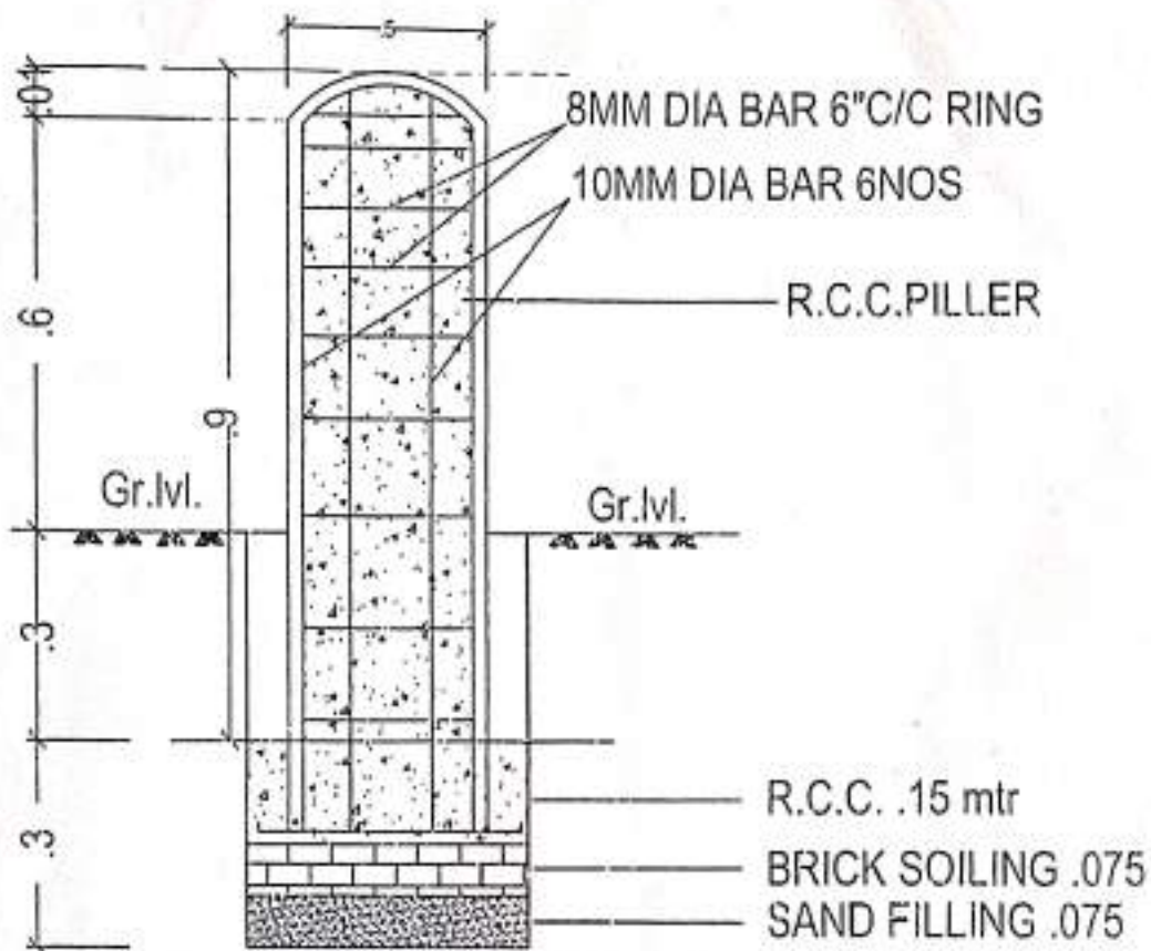
CROSS SECTION OF PILLER UNIT IN METER
