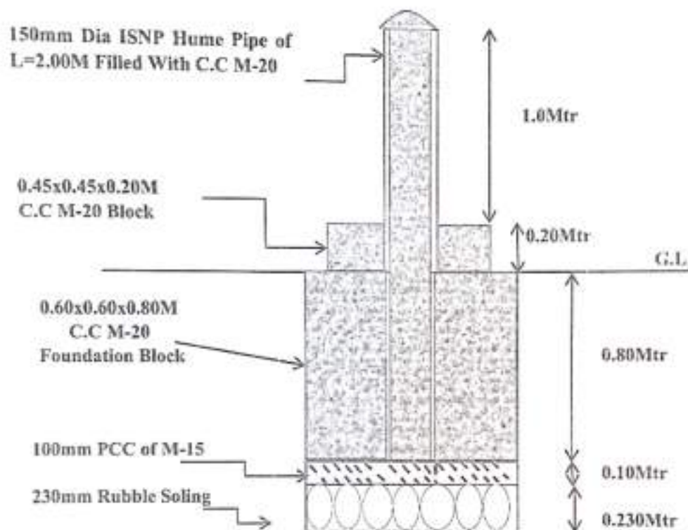
SECTIONAL VIEW OF BOUNDARY DEMARCTION PILLAR
