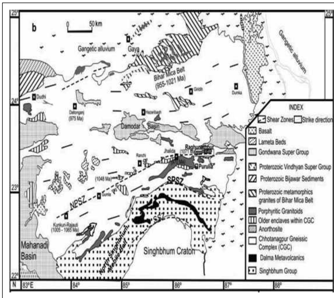
Figure-6.4: Geological map of the Chhotanagpur Gneissic Complex (CGC)( After Basu1993)
