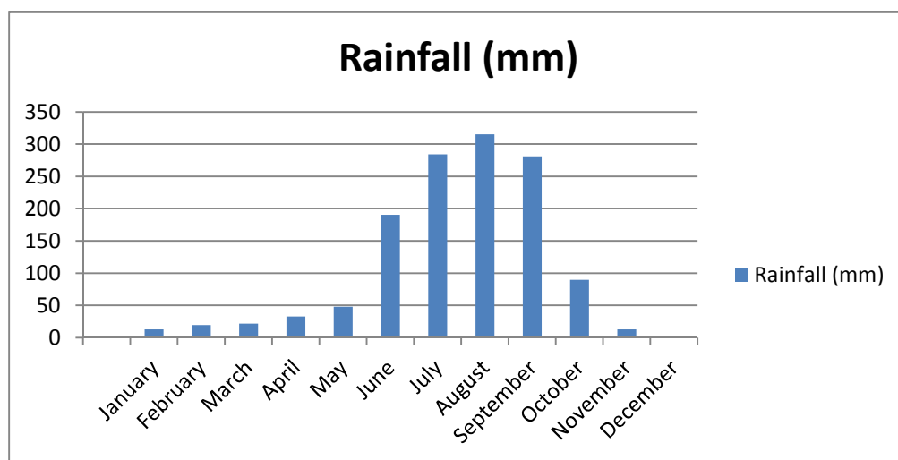
Figure-6.1: Monthwise Variation of Rainfall in Project Area District
