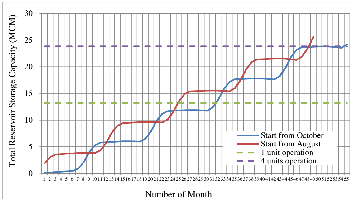
Figure-5.7 Impounding Schedule for Average Year (with environmental flow)
