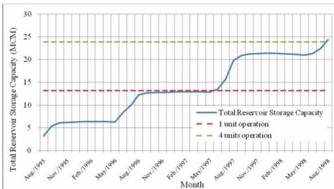
Figure-10.1: Impounding Schedule for Wet Years (with Environmental Flows)
