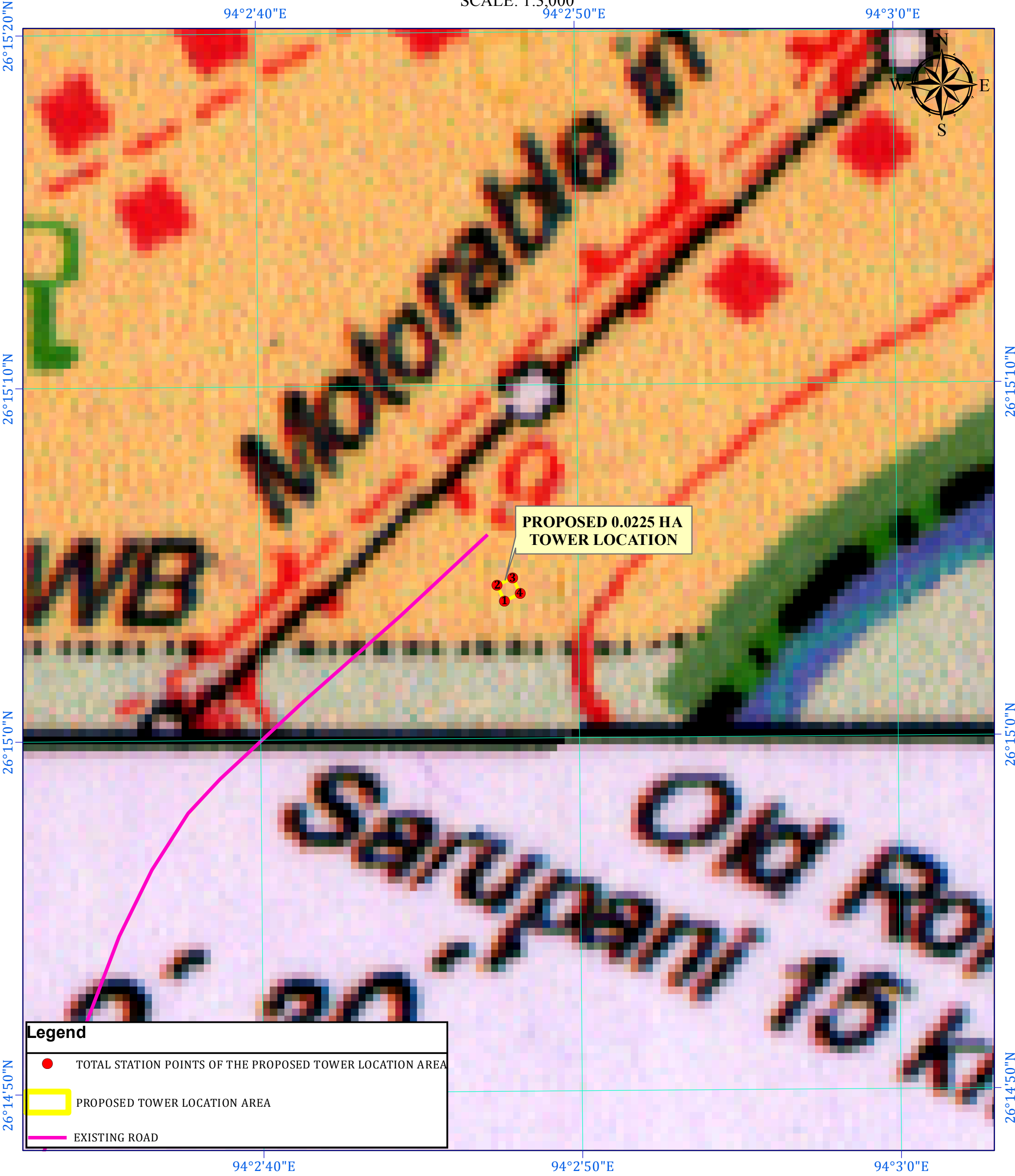
TOTAL STATION COORDINATE READINGS
