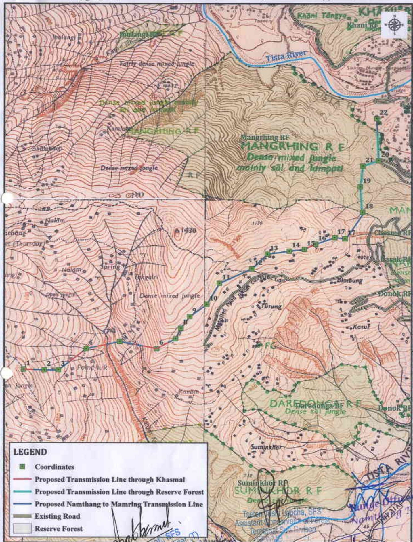
MAP SHOWING THE LOCATION FOR CONSTRUCTION OF 66KV D/C NAMTHANG- MAMRING (18 M) CORRIDOR PASSES THROUGH GOVT. KHAMAL (1.8216 Ha) / RESERVE FOREST (AREA: 17136 SQM OR 1.7136 HA) UNDER NAMTHANG (T) RANGE, SOUTH SIKKIM.
