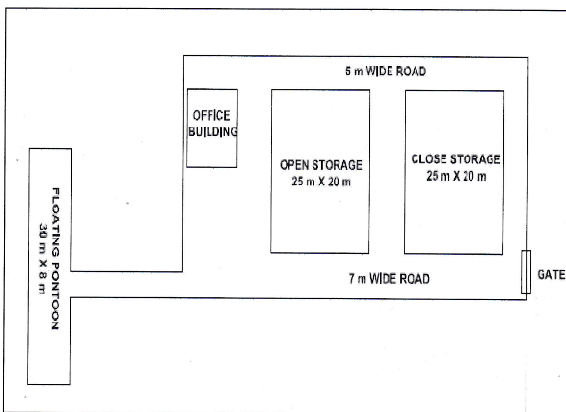
Terminal Layout Plan at Demagiri
