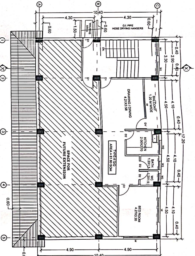
THIRD FLOOR PLAN 88 SQM.
