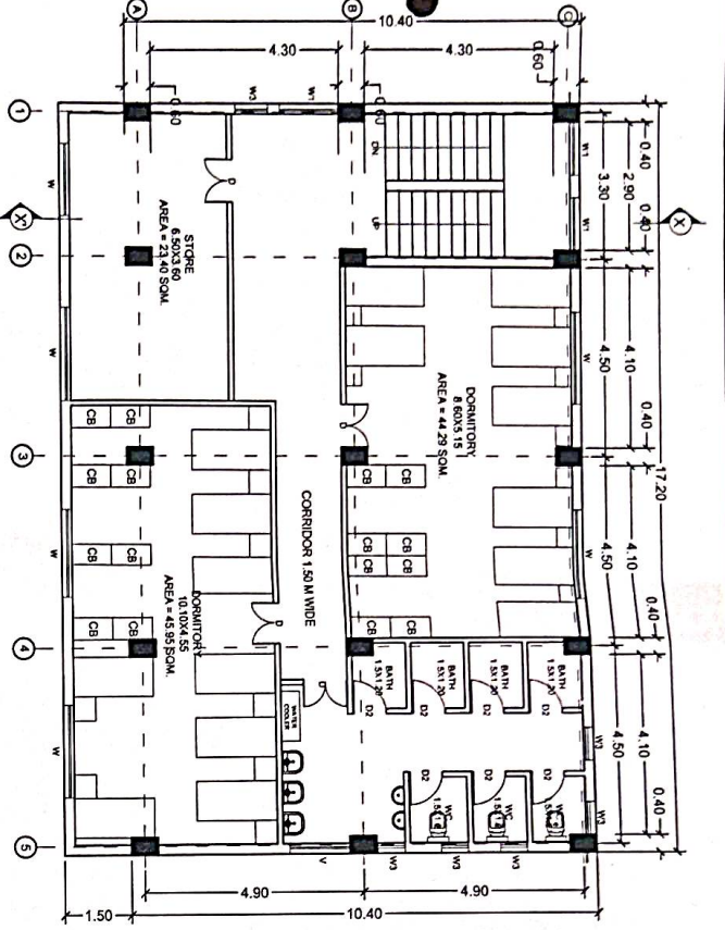
SECOND FLOOR PLAN 205 SQM.
