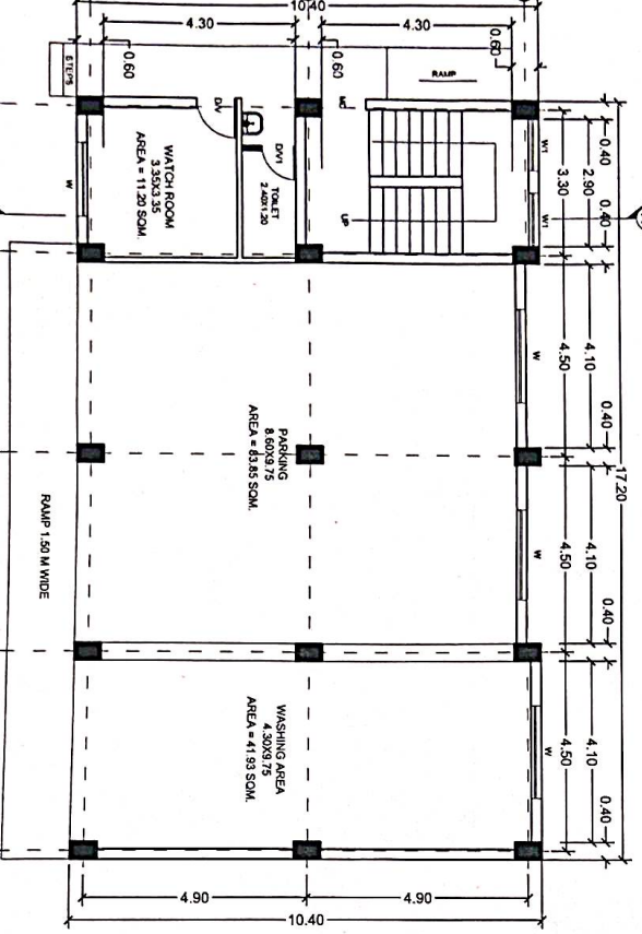
GROUND FLOOR PLAN 179 SQM.
