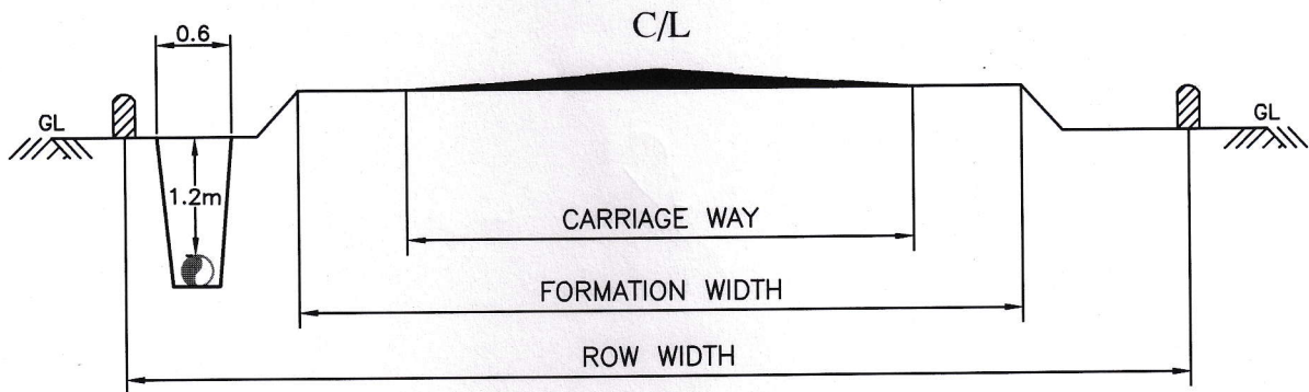
CROSS SECTION OF ROAD
