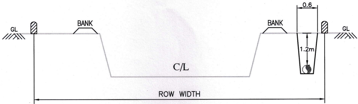
CROSS SECTION OF CANAL
