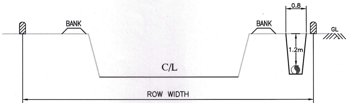
CROSS SECTION OF CANAL
