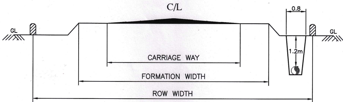
CROSS SECTION OF SH
