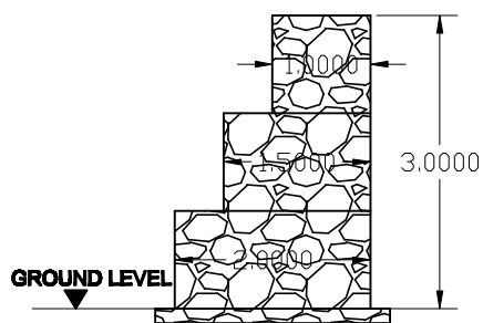
Cross Section of Gabion Wall(3.0M HT.)
