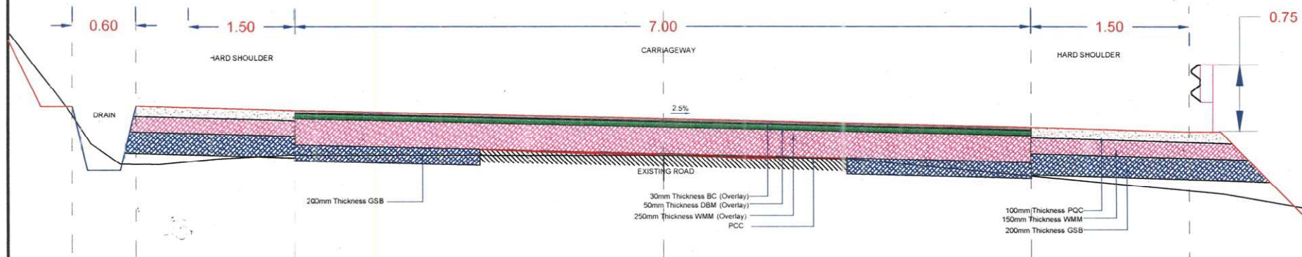
TYPICAL CROSS SECTION-1 OPEN SECTION
