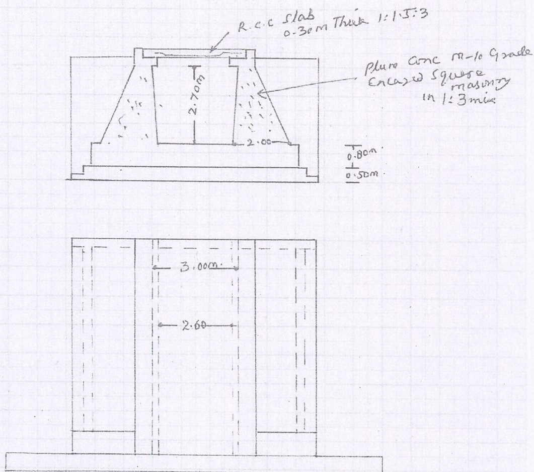
PLAN 3m span R.C.C. Culvert.
