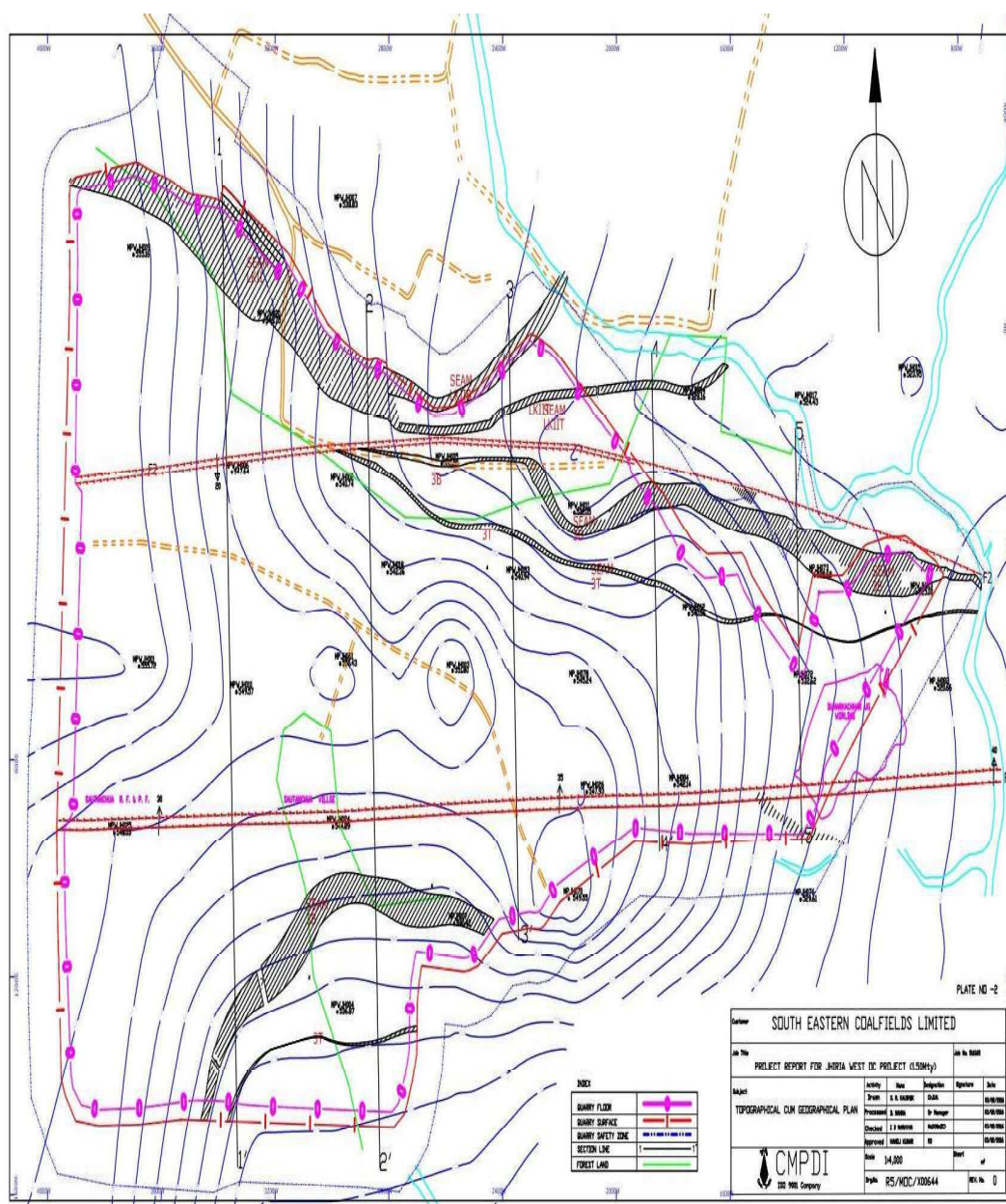
Topographical Plan
