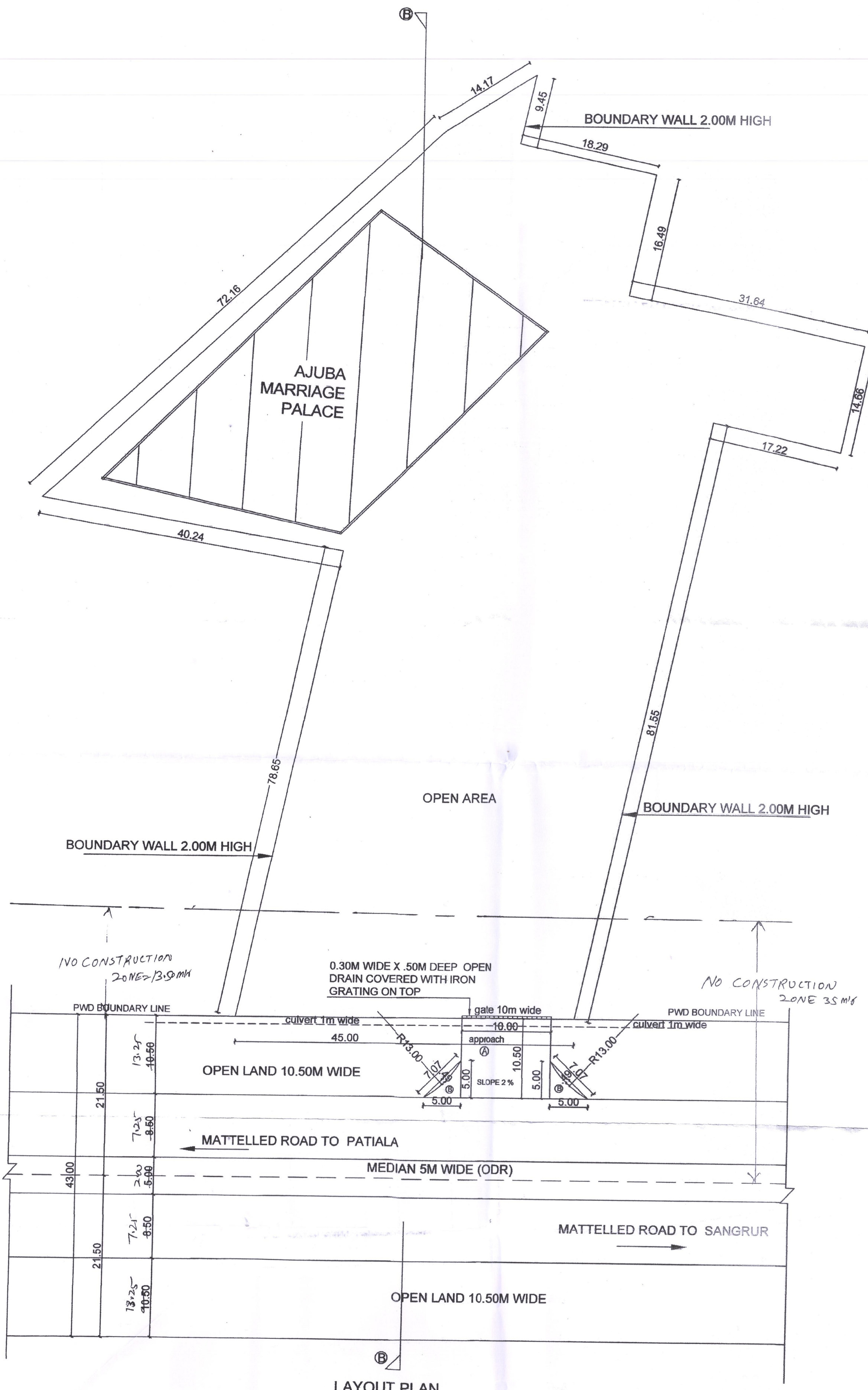
LAYOUT PLAN
