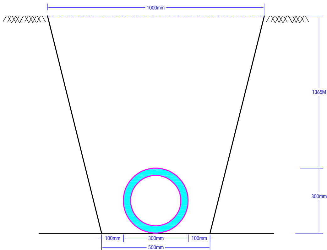
TYPICAL TRENCH SECTION FOR LAYING STEEL (300 mm Ø)
