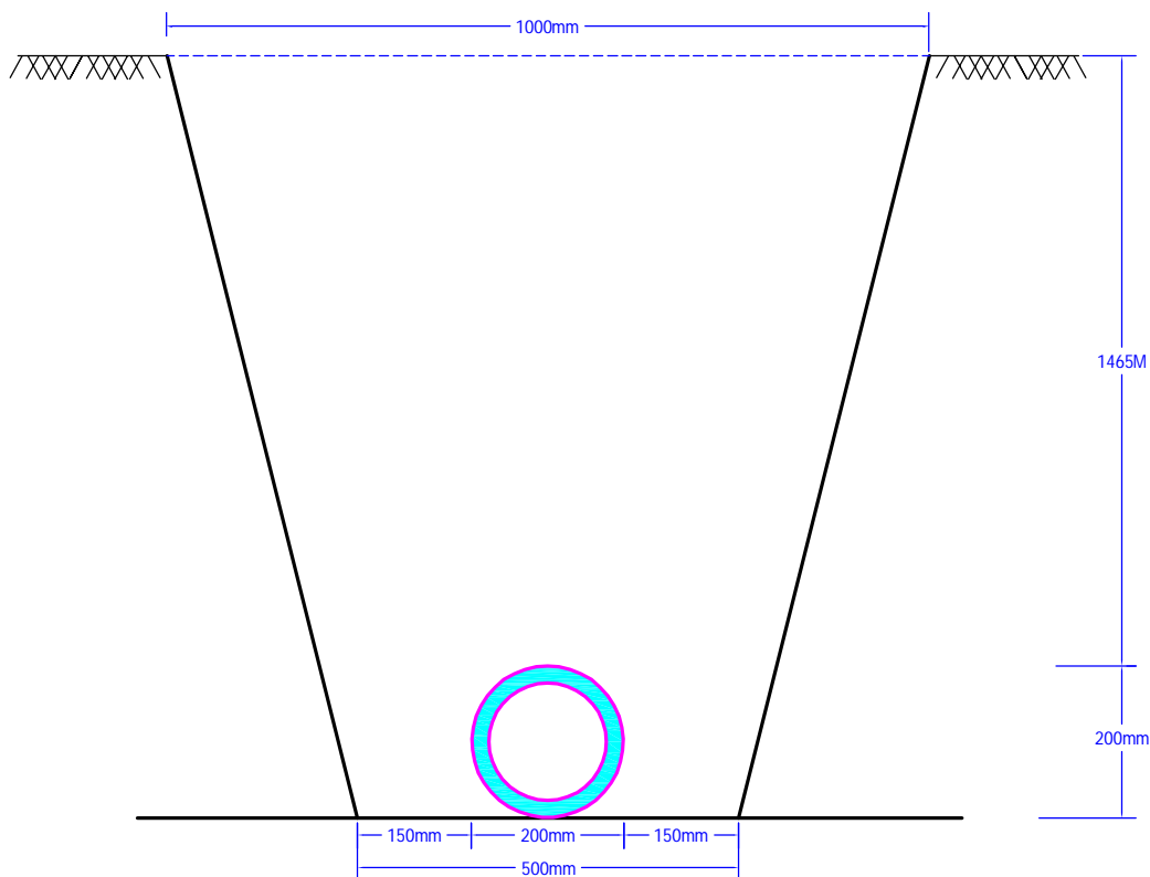
TYPICAL TRENCH SECTION FOR LAYING STEEL (200 mm Ø)
