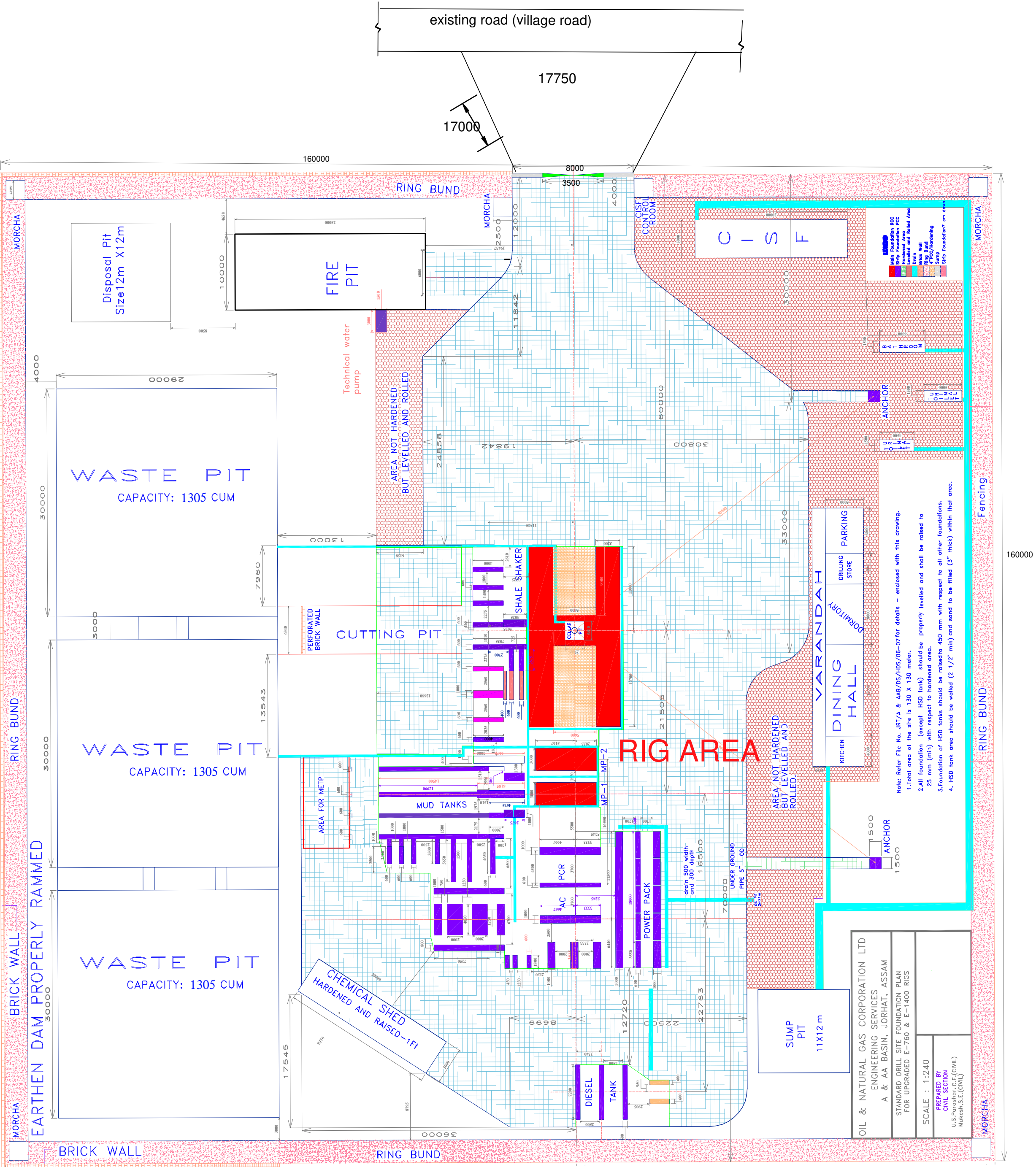
DETAILED LAYOUT PLAN
