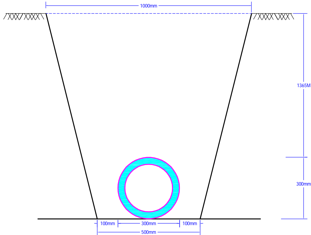
TYPICAL TRENCH SECTION FOR LAYING STEEL (300 mm Ø)
