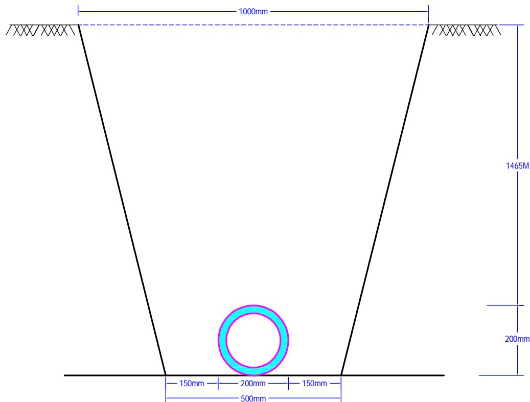
TYPICAL TRENCH SECTION FOR LAYING STEEL (200 mm Ø)
