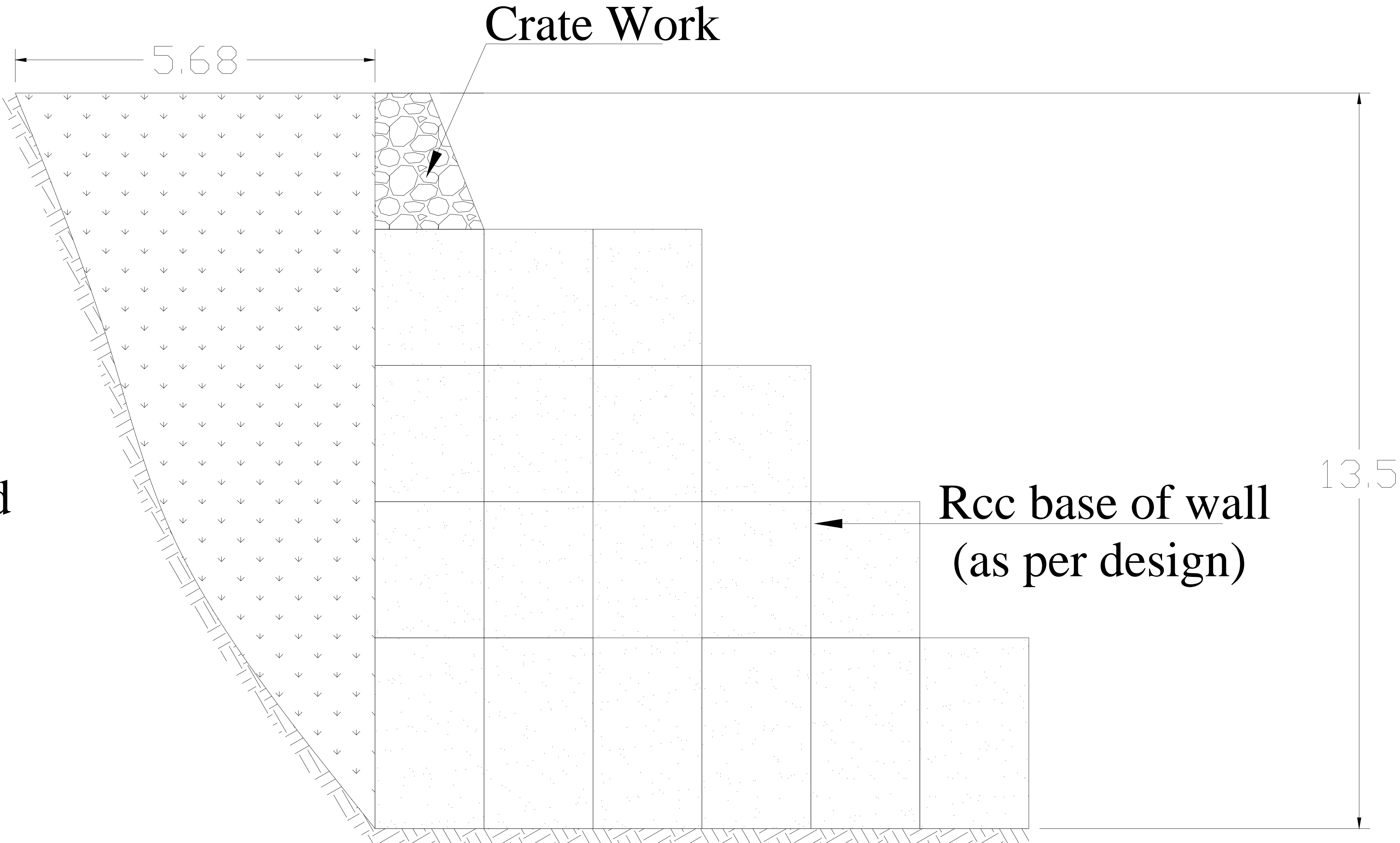
Section at Y-Y
