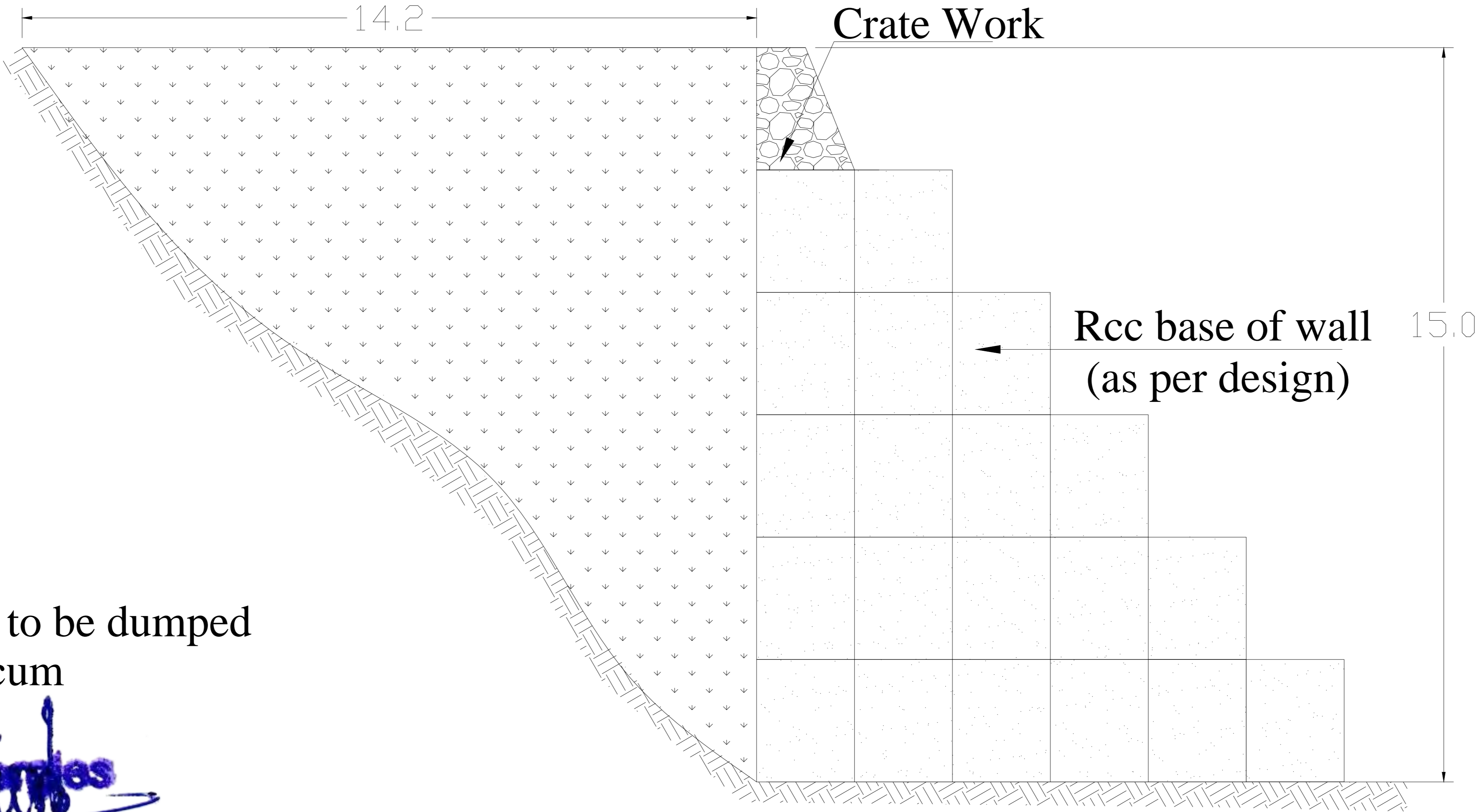
Section at X-X (Cross-section)
