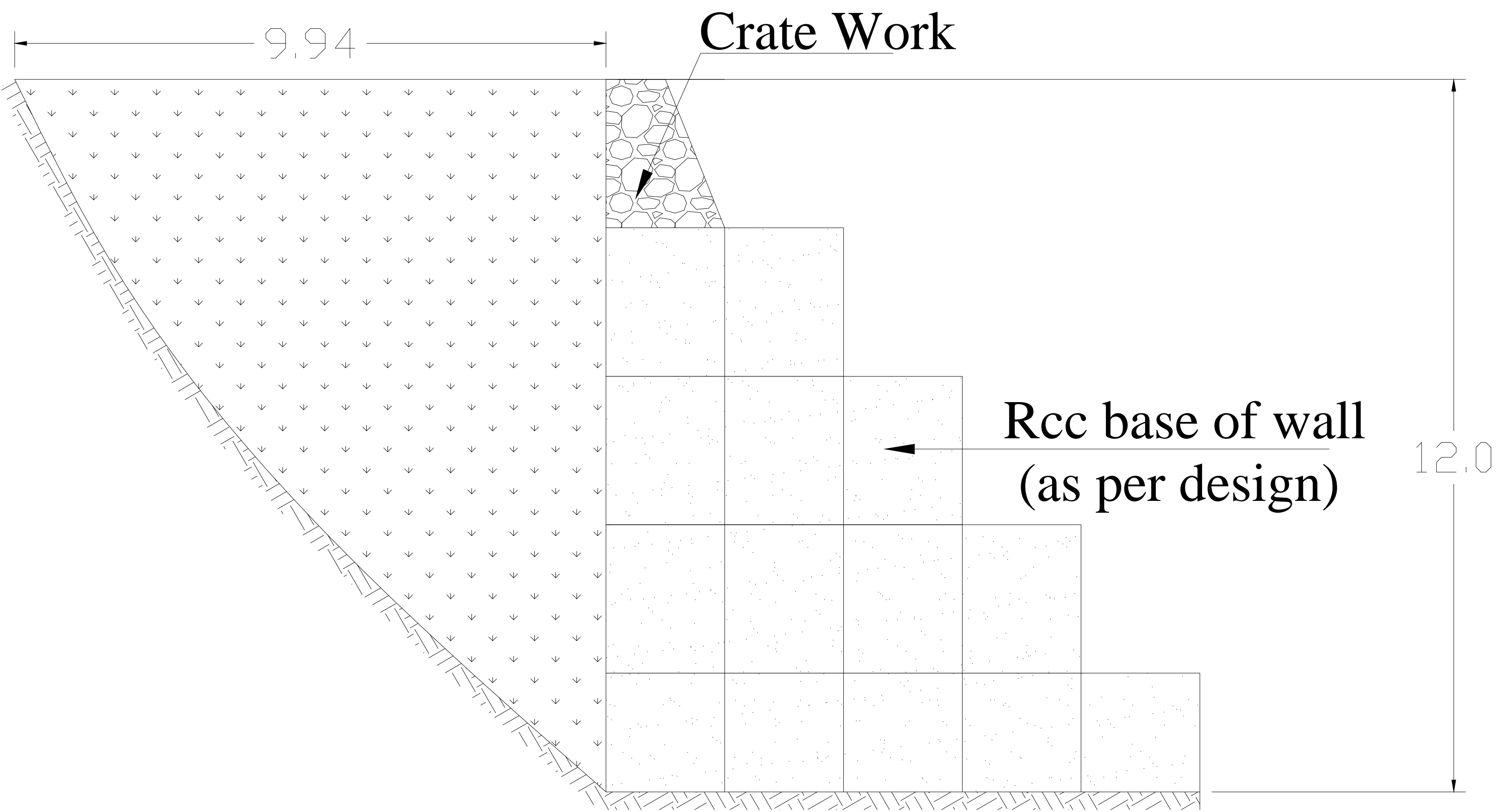
Section at X-X (Cross-section)
