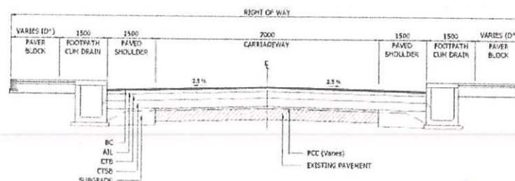
TCS-2 - RECONSTRUCTION + WIDENING IN URBAN SECTION
