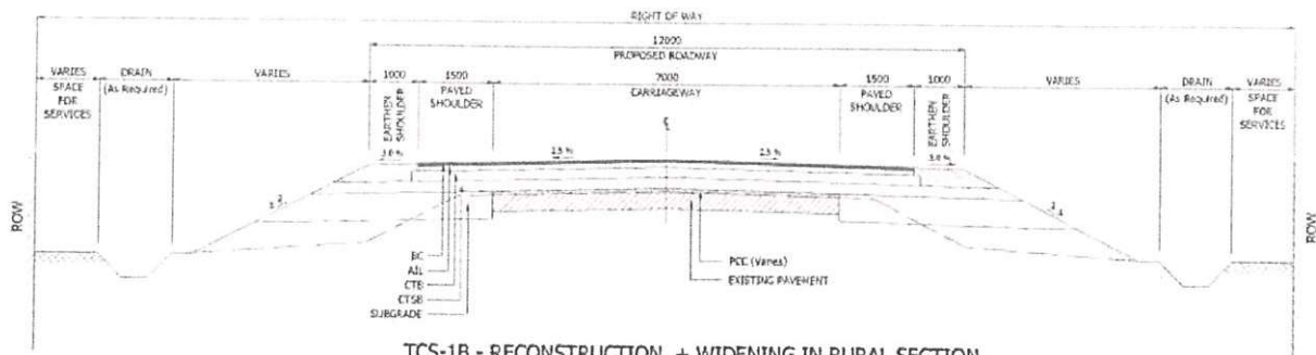
TCS-1B - RECONSTRUCTION + WIDENING IN RURAL SECTION
