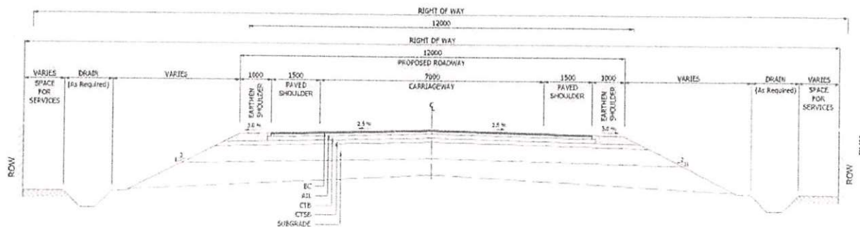
TCS-1A - NEW CONSTRUCTION + REALIGNMENT / BYPASS IN RURAL SECTION
