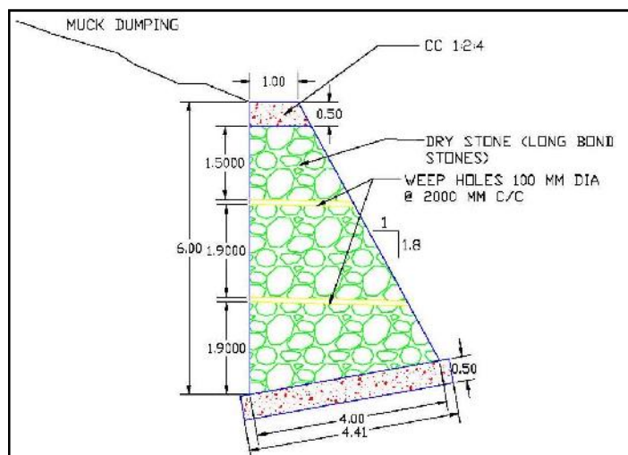
Figure 4: Cross Sections of the proposed retaining wall
