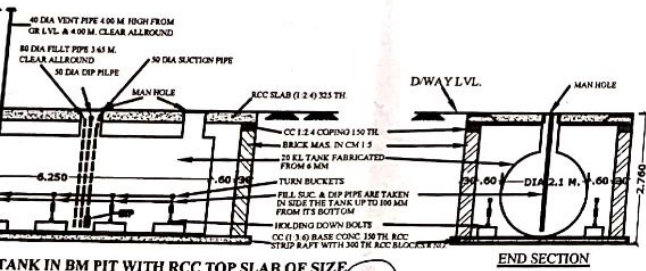
END SECTION
