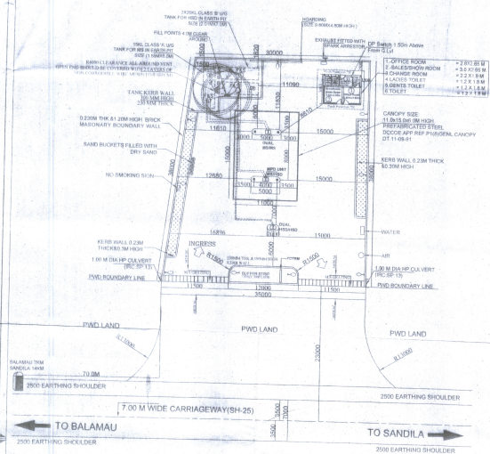
LAYOUT PLAN SCALE 1:250
