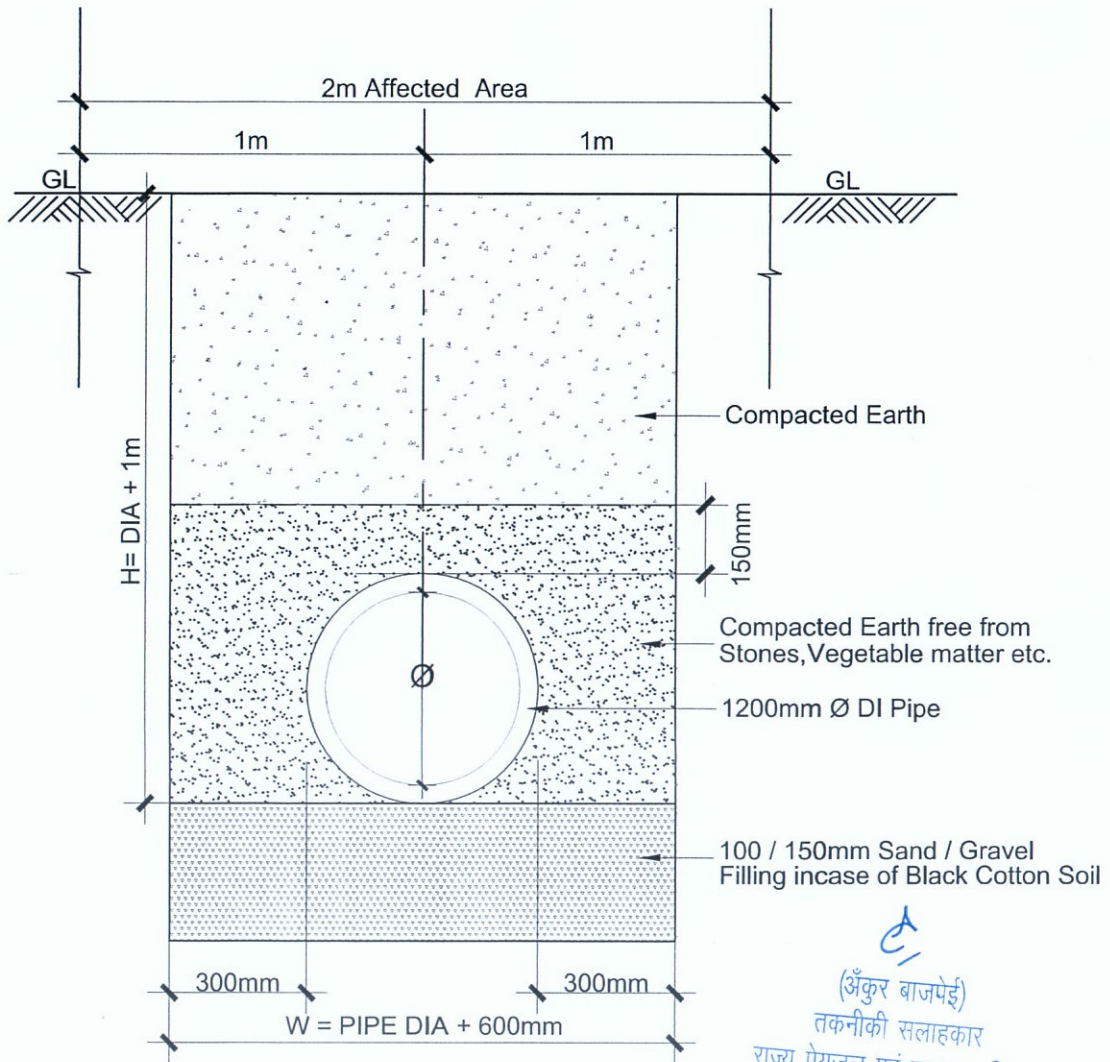
Typical Detail of Trench
