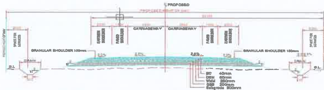
TCS-2 2-LANE CARRIAGEWAY WITHOUT SERVICE ROAD NEW CONSTRUCTION
