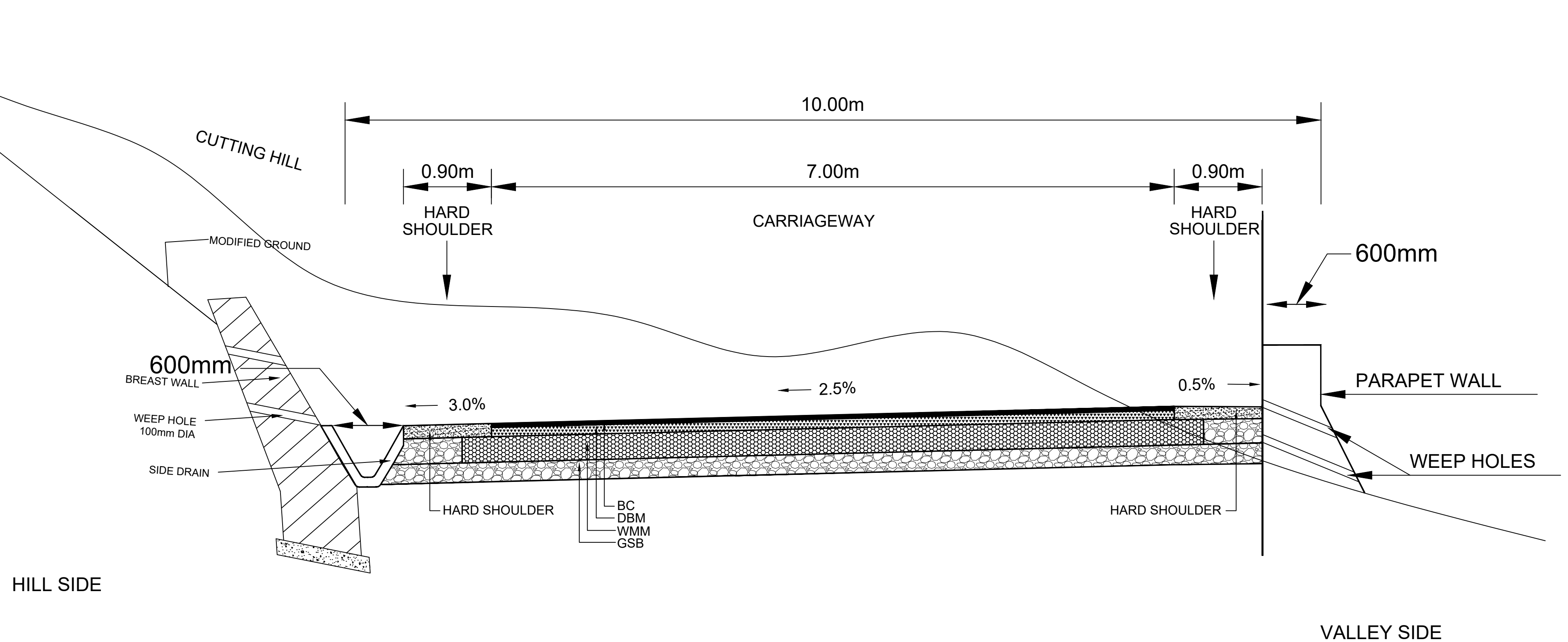
TCS NO.6 REALIGNMENT ON HILL SIDE WITH BREAST WALL (LHS HILL)
