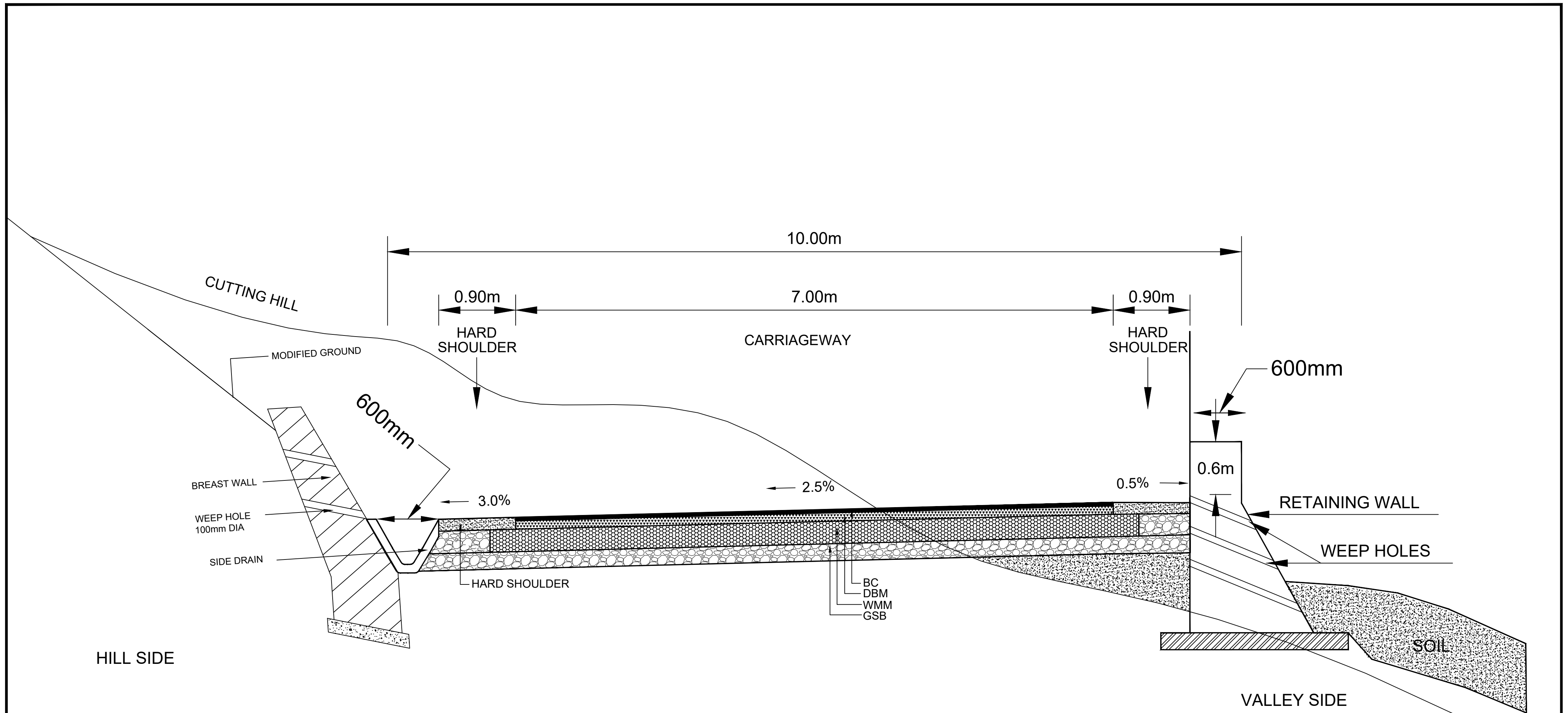
TCS NO.12 REALIGNMENT WITH RETAINING & BREAST WALL (LHS HILL)
