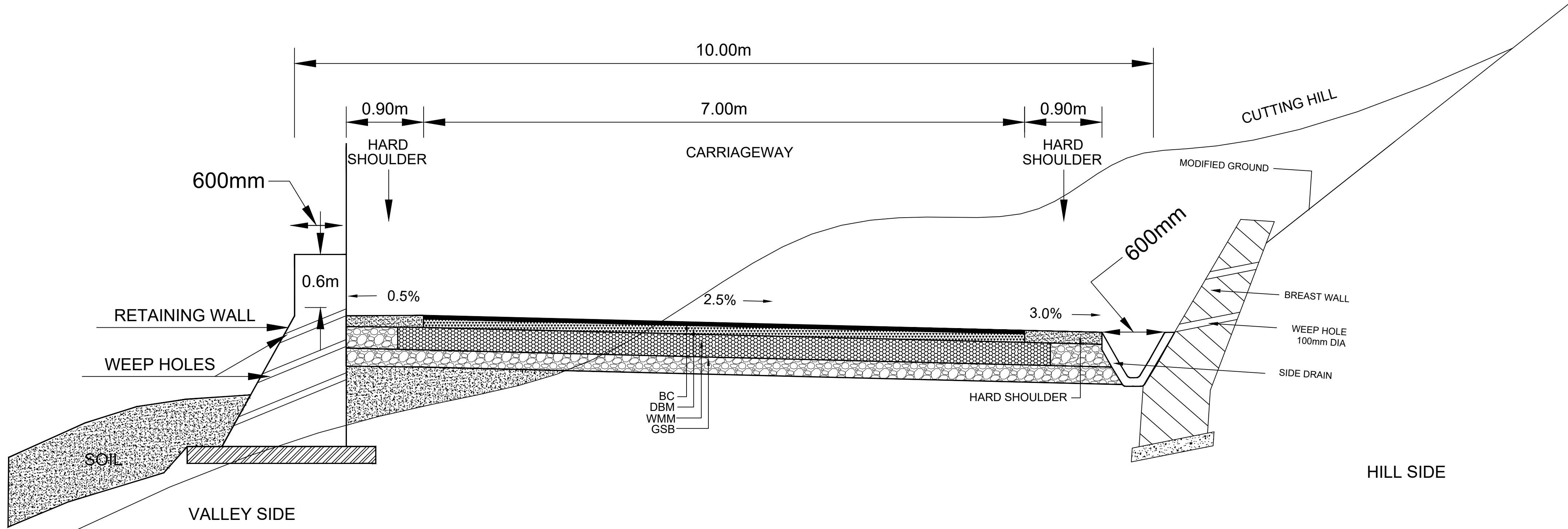
TCS NO.11 REALIGNMENT WITH RETAINING & BREAST WALL (RHS HILL)
