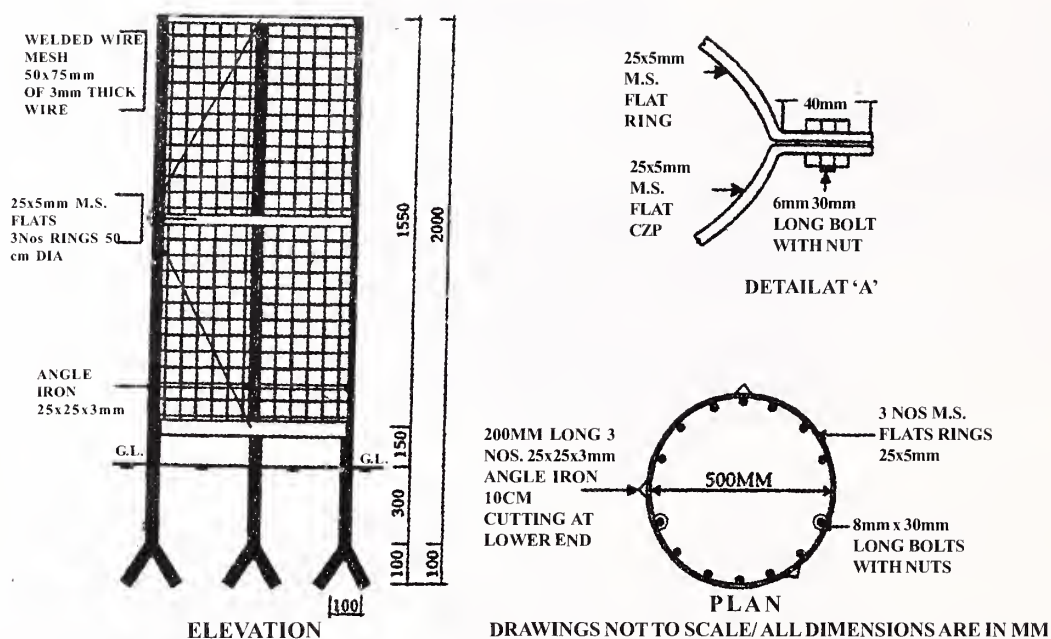
Fig. 31 Ornamental Tree Guard with Welded Mesh
