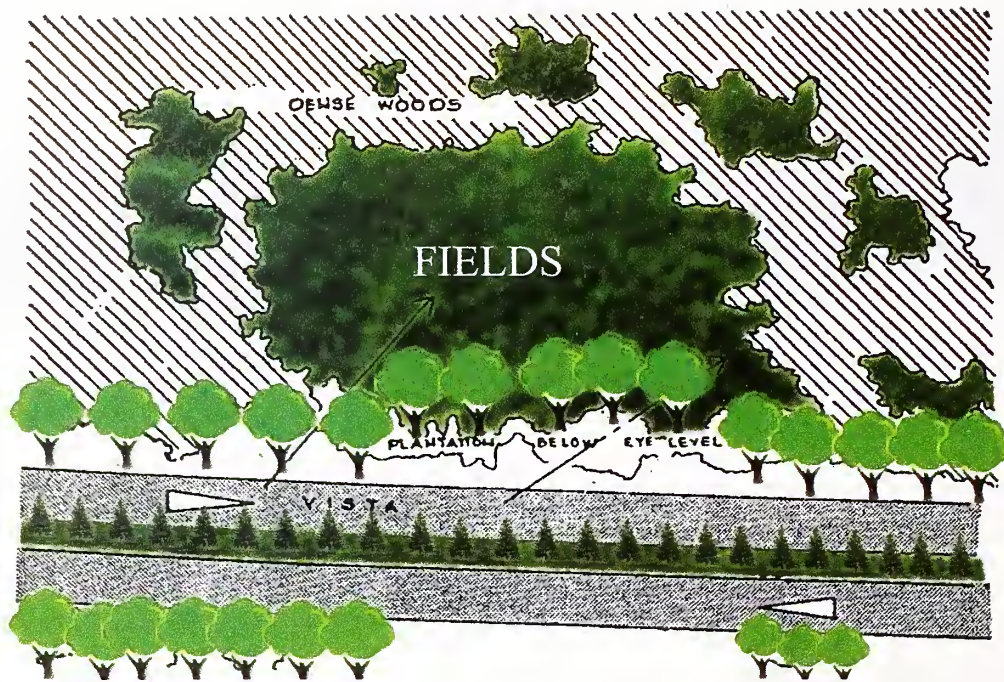
Fig. 28 Exposing Scenic Spots and Open Vistas in Continuously Wooded Areas through Selective Pruning of Plantation
