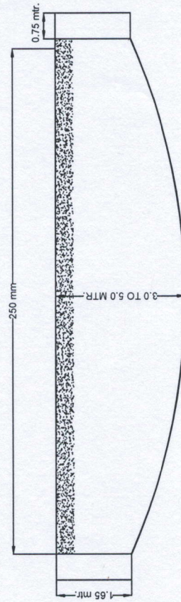
CROSS SECTION VIEW OF HDD SHOT
