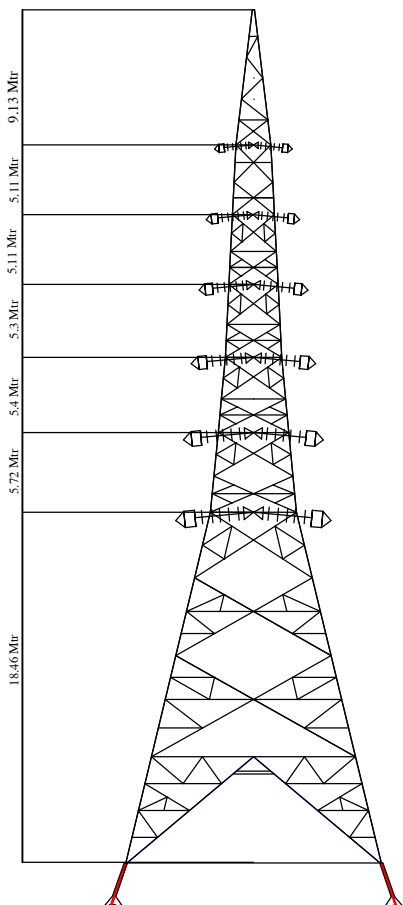
Multicircuit tower diagram
