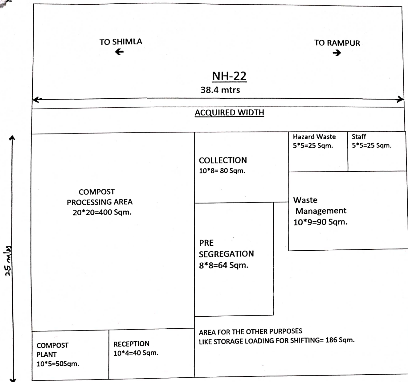
SITE PLAN FOR THE MSW PROJECT AT KHASRA NO. 268/1 AT MAUJA M.M JANGLE D-52 ROHRU THEOG(SHIMLA) AREA 960 Sqm.
