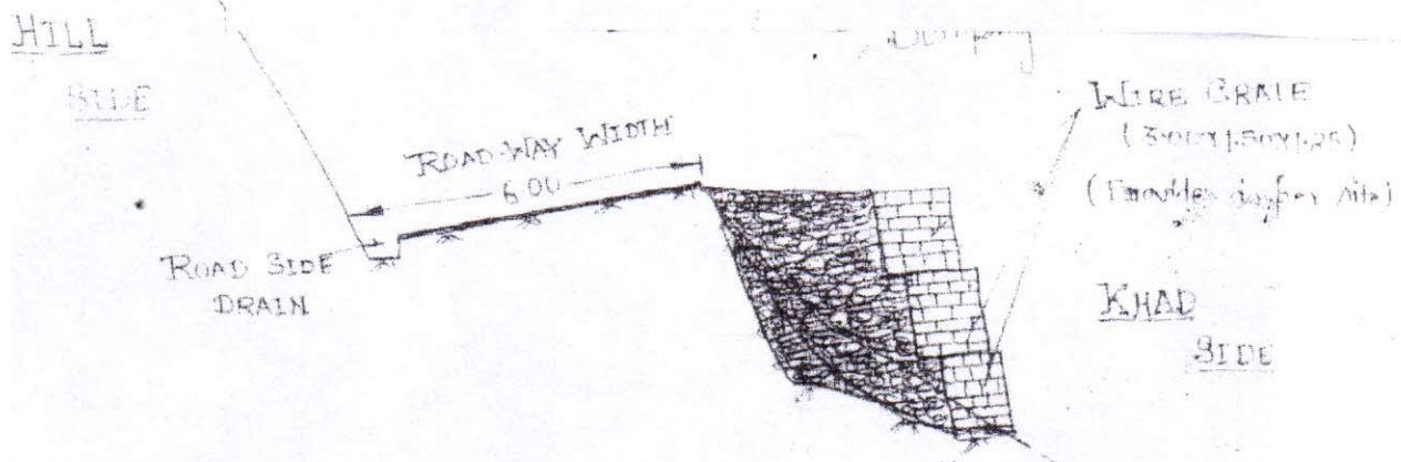
TYPICAL X-SECTION
