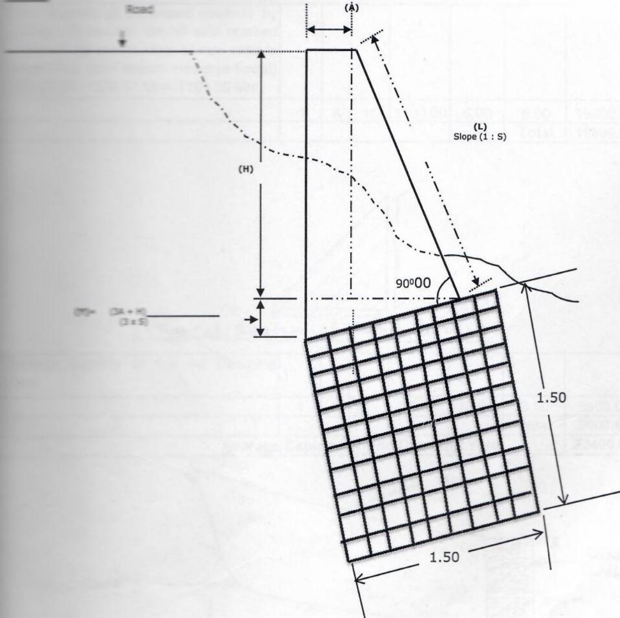
Retaining Wall With Wire Crate
